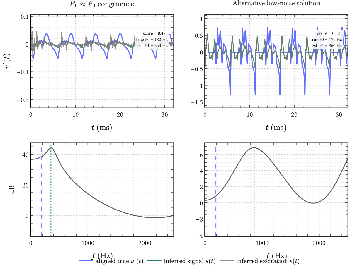
Figure 40 | Two failure modes from the BNGIF benchmark. Top: aligned true DGF (blue), inferred structured signal s(t) (green), and inferred excitation e(t) (grey). Bottom: inferred AR envelope with true F_0 (dashed blue) and estimated \hat{F}_1 (dotted green). Left: F_1 \approx F_0 congruence – the filter absorbs the fundamental, flattening the excitation. Right: the model finds an alternative low-noise decomposition with the wrong source shape.
