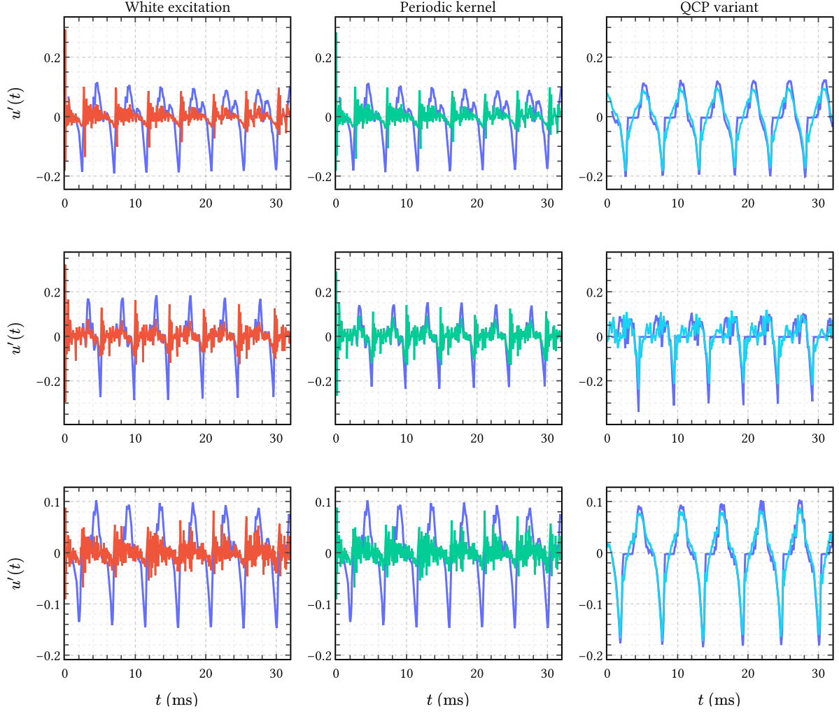
Figure 7 | Three representative EGIFA speech frames. In each panel, the blue curve is the aligned true DGF u'(t) and the colored curve is the estimated excitation. Left: white excitation. Center: Yoshii and Goto’s periodic kernel. Right: the QCP variant. The first row shows the typical case: periodic structure helps, but only modestly. The second row shows a frame where the periodic kernel already gives a clearly better voiced fit than white excitation. The third row shows the real failure mode: both vanilla IKLP variants still miss badly, while the QCP variant locks onto the closure pattern.
