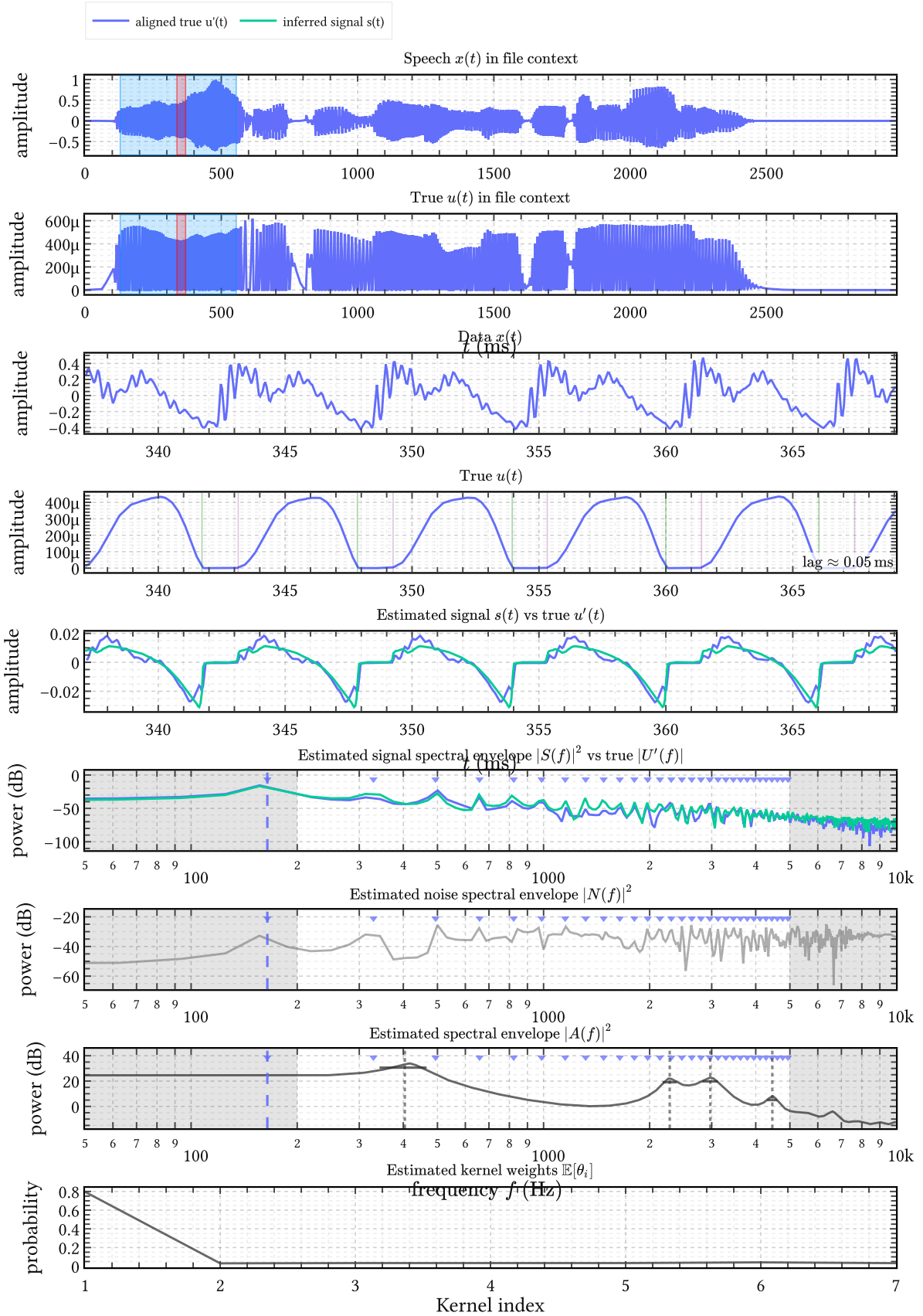
Figure 39 | Representative BNGIF estimate from the EGIFA benchmark. Full-file context is shown at top left; the selected analysis frame appears directly below. In the main source panel, the inferred structured signal s(t) is compared against the aligned true DGF u'(t) . The spectral panels show the corresponding source, noise, and AR-envelope decomposition, while the kernel-weight panel shows which learned source hypotheses are active in the fit
