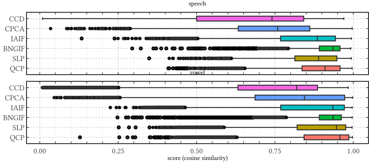
Figure 37 | EGIFA benchmark scores by method and collection. Scores are centered cosine similarities after affine+lag alignment (Appendix E). The classical baselines are CPCA, CCD, IAIF, SLP, and QCP; the Bayesian result is BNGIF. On speech, BNGIF leads; on vowels, QCP remains strongest.
