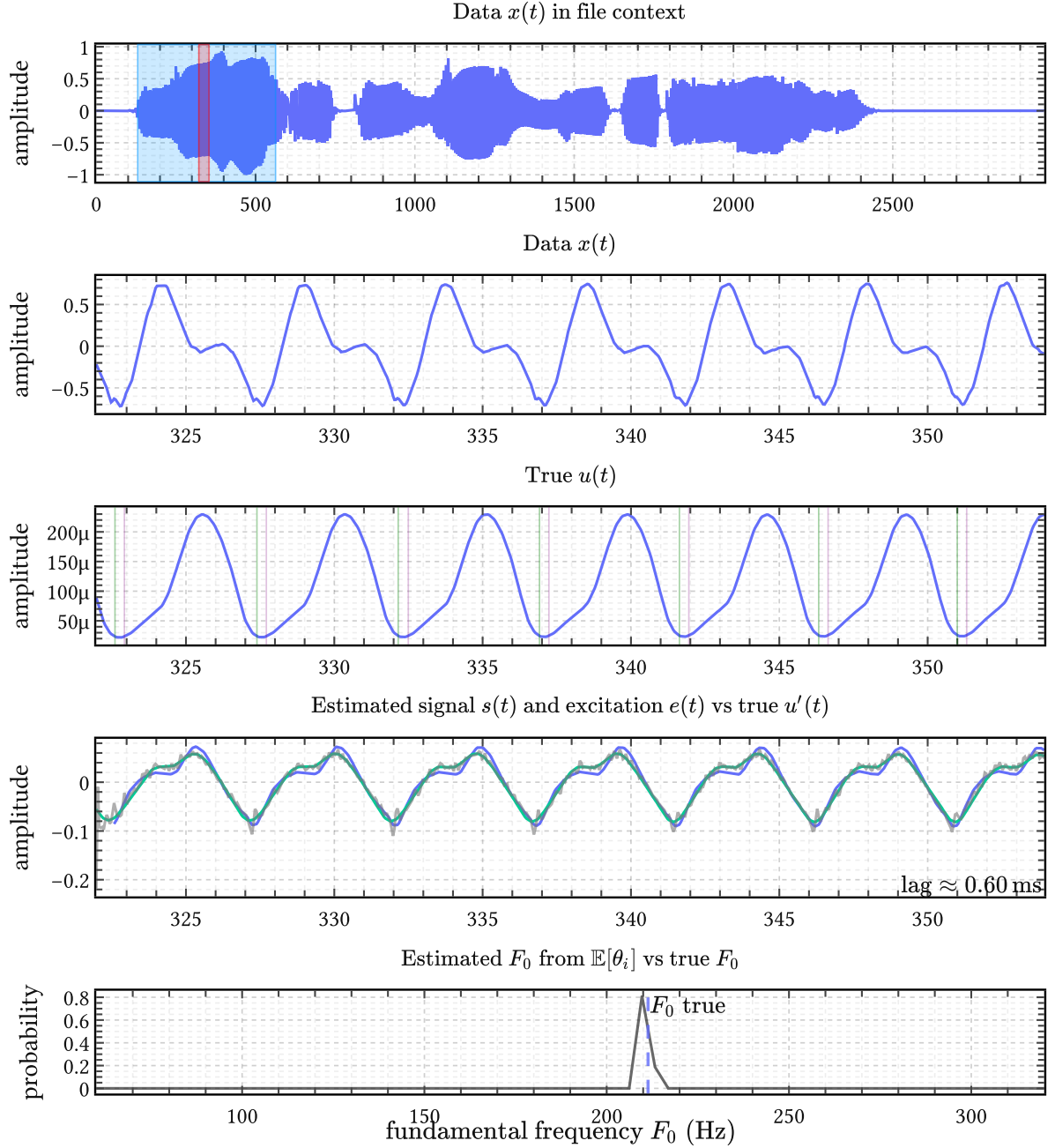
Figure 5 | One periodickernel IKLP fit in detail. Top: the analyzed EGIFA speech file and the selected 32 ms frame. Middle: the frame-local speech signal, the aligned true DGF u'(t) , and the inferred structured signal s(t) together with the full excitation estimate \varepsilon(t) . Bottom: the posterior over candidate F_0 values derived from \mathbb{E}[\theta_i] . The intended mechanism is already visible: weight mass concentrates near one fundamental frequency and the excitation estimate is pulled toward that periodic structure while the tract envelope is fitted jointly.
