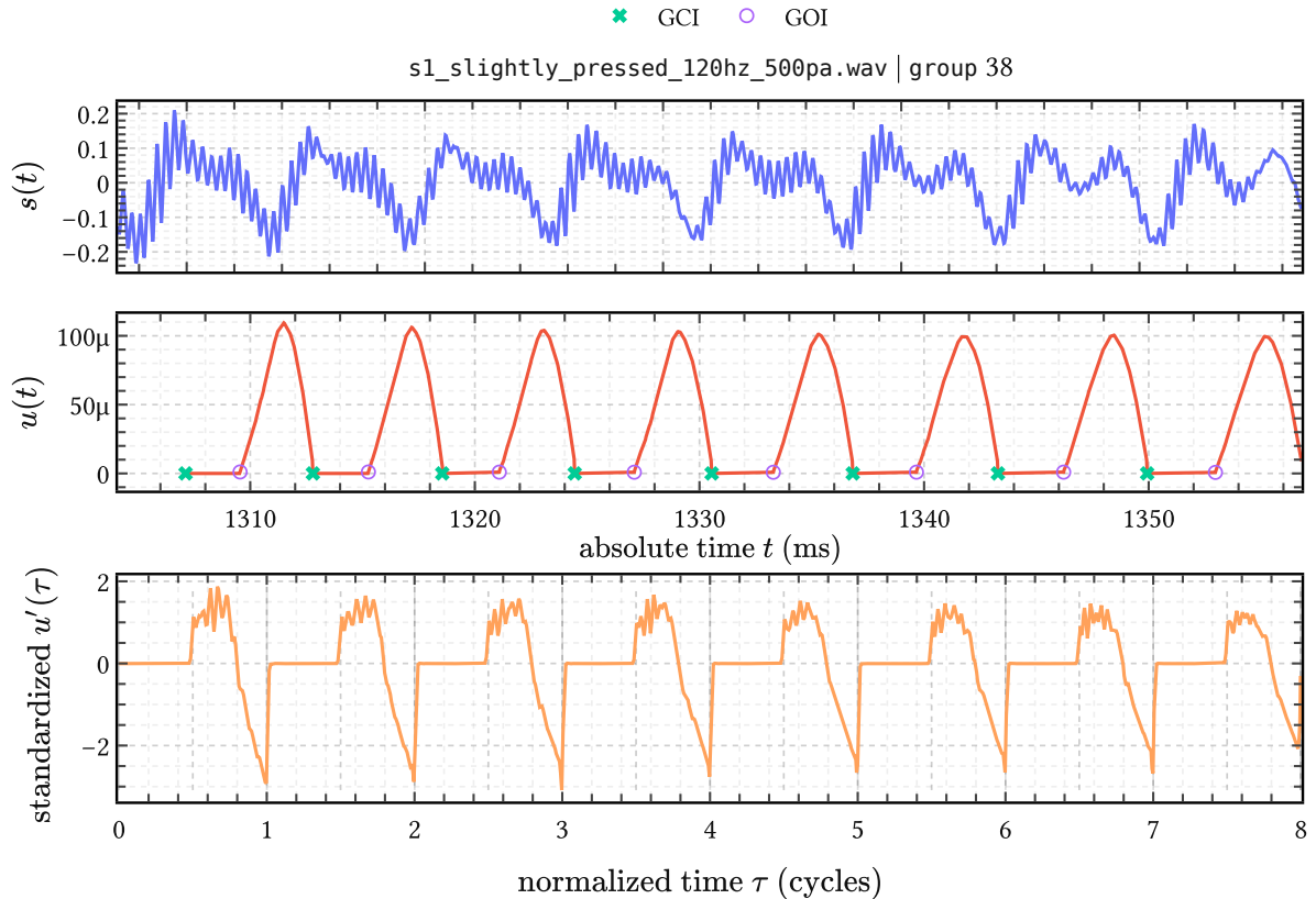
Figure 42 | Registration of one EGIFA voiced group. Top: raw speech s(t) in physical time. Middle: raw glottal flow u(t) with LBGID-detected GCI and GOI events. Bottom: the group after differentiation, normalization, and warp to normalized time \tau , shown as u'(\tau) ; GCIs at integers, GOIs at half-integers.
