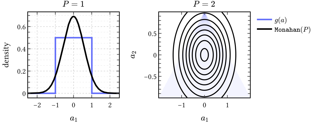
Figure 9 | Geometry mismatch. For P = 1 the Monahan map is just a_1 = \varphi_1 and \mathcal{A}_1 = (-1, 1) . For P = 2 it gives (a_1, a_2) = (\varphi_1(1 - \varphi_2), \varphi_2) , so uniform PACF draws induce a density g(\mathbf{a}) supported on the triangular stable region. The Monahan prior \text{Monahan}(P) matches the first two moments of g , but it cannot reproduce the bounded, non-elliptical shape of that support faithfully, and mass leaks out of the region of stable filters.
