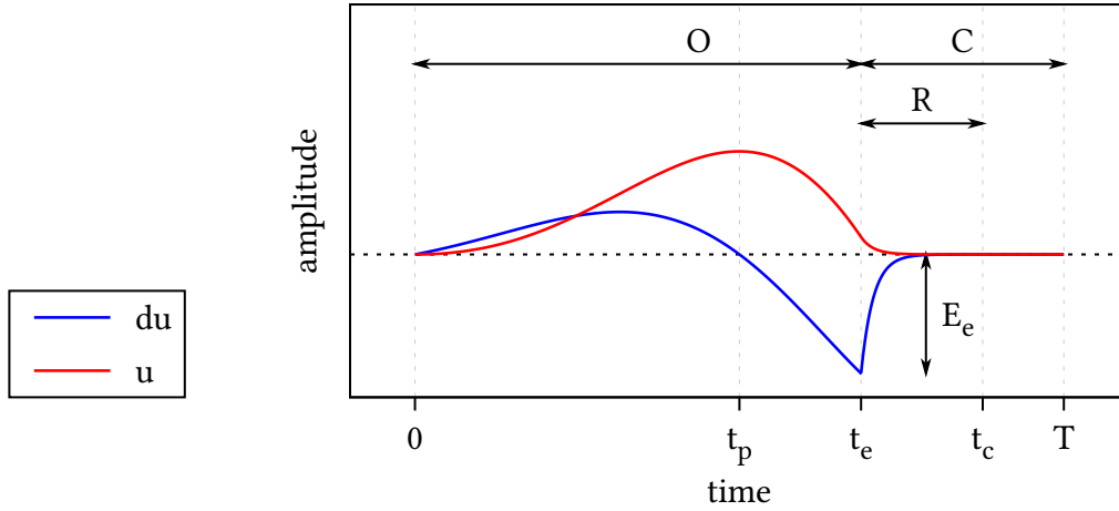
Figure 8 | The Liljencrants-Fant model for \text{—} u'_{\text{LF}}(t) and \text{—} u_{\text{LF}}(t) during a single period of length T . The open phase (O), closed phase (C) and return phase (R) are marked at the top and are determined by the changepoints \{t_p, t_e, t_c, T\} . The amplitude at peak excitation t_e is E_e . Not shown here is time constant of the return phase T_a , which during (R) determines the steepness of exponential decay towards zero in u'(t) .
