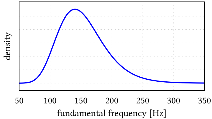
Figure 14 | Analytic marginal fundamental frequency distribution implied by the log-period prior. The distribution is lognormal with median 150 Hz, 5-95% range approximately 100-224 Hz (2.5-97.5%: 92-244 Hz).
