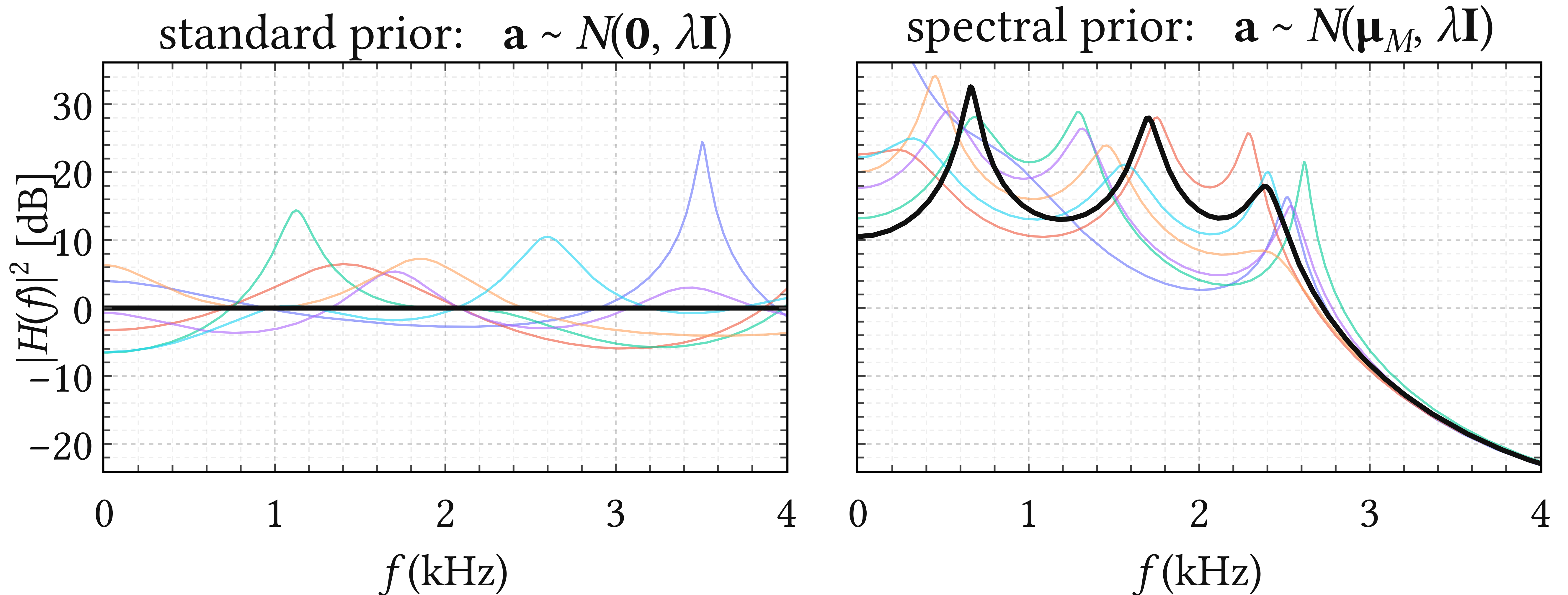
Predicted envelopes |H(f)|^2 under each prior; bold: prior mean; dotted: the three resonances given to the spectral prior. More examples behind the QR code.
