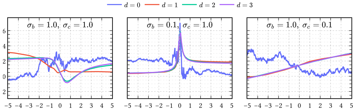
Figure 21 | Prior samples from TACK for different degrees d . Each column fixes a different covariance setting (\sigma_b, \sigma_c) . Within each column the four curves correspond to different values of d . Increasing d progressively softens the hinge-point-like behavior, while decreasing \sigma_b relative to \sigma_c makes the prior more localized around the center.
