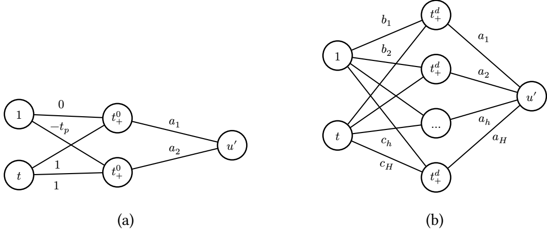
Figure 20 | Neural network view. (a) The triangular pulse model as a tiny neural network with a single hidden layer, linear readout and t_+^0 activation. (b) The general parametric polynomial model of degree d with order H with hidden weights \{\mathbf{b}, \mathbf{c}\} \in \mathbb{R}^{2H} , output weights \mathbf{a} \in \mathbb{R}^H and RePU activation function t_+^d .
