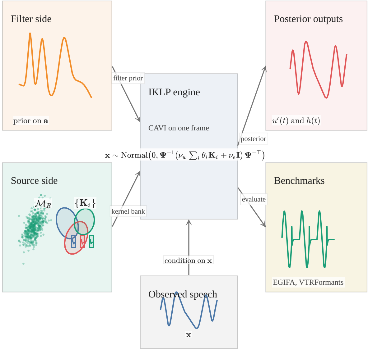
Figure 41 | Assembly of BNGIF from the learned source mixture and IKLP. The refined surrogate mixture \mathcal{M}_R is first mean-folded into zero-mean source kernels \mathbf{K}_i . These are then combined with the AR operator \Psi and inferred by CAVI under the IKLP model.
