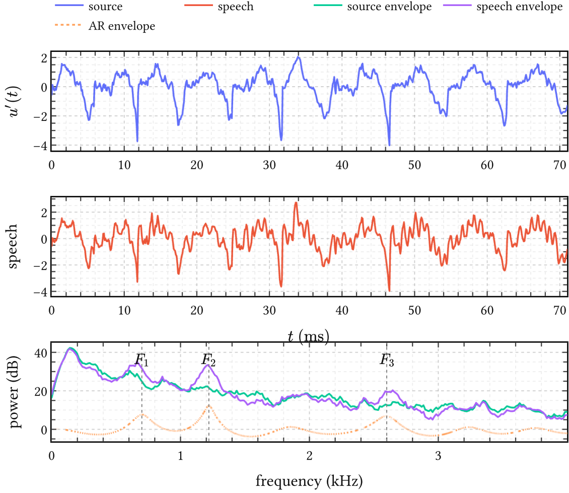
Figure 40 | Generated voiced speech fragment. Top: source waveform u'(t) obtained by drawing \mathbf{u}' \mid \boldsymbol{\tau}, \mathcal{M}_R and transporting it through the warp induced by \mathcal{P} . Middle: speech waveform after applying the AR filter with coefficients from (177), conditioned on an open-vowel formant pattern. Bottom: spectral envelopes of source and speech together with the AR envelope; F_1, F_2, F_3 targets are marked.
