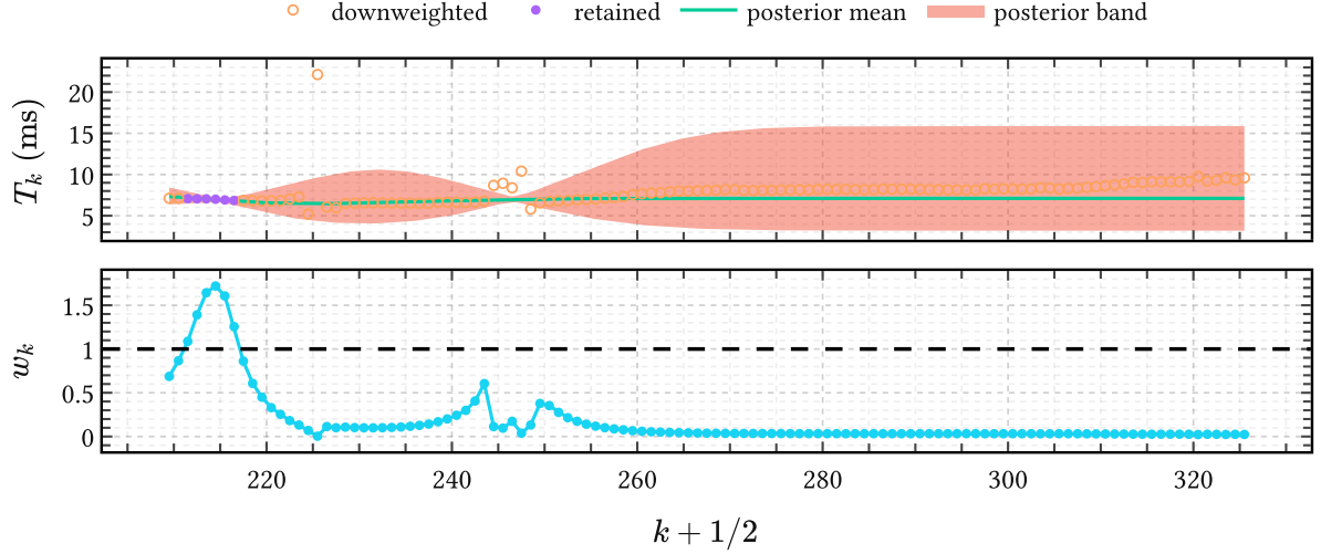
Figure 33 | t-PRISM on an inter-GCI period track. The top panel shows a local EGIFA period sequence together with the t-PRISM posterior mean and uncertainty band learned from the APLAWD pitch-track prior. The bottom panel shows the inferred precision weights w_k = \mathbb{E}[\lambda_k] for the same excerpt. When the observed periods deviate sharply from the smooth local trend, their weights collapse below one and they are automatically downweighted rather than fitted.
