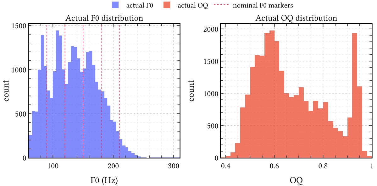
Figure 30 | Implied F_0 and OQ distributions from LBGID landmarks on EGIFA. Left: the frame-level F_0 distribution implied by the detected GCIs, with dashed lines indicating EGIFA's nominal pitch settings. Right: the corresponding frame-level OQ distribution implied by the detected GCI/GOI pairs.
