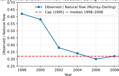
Murray River at Swan Hill: flow reduction during Millennium I
