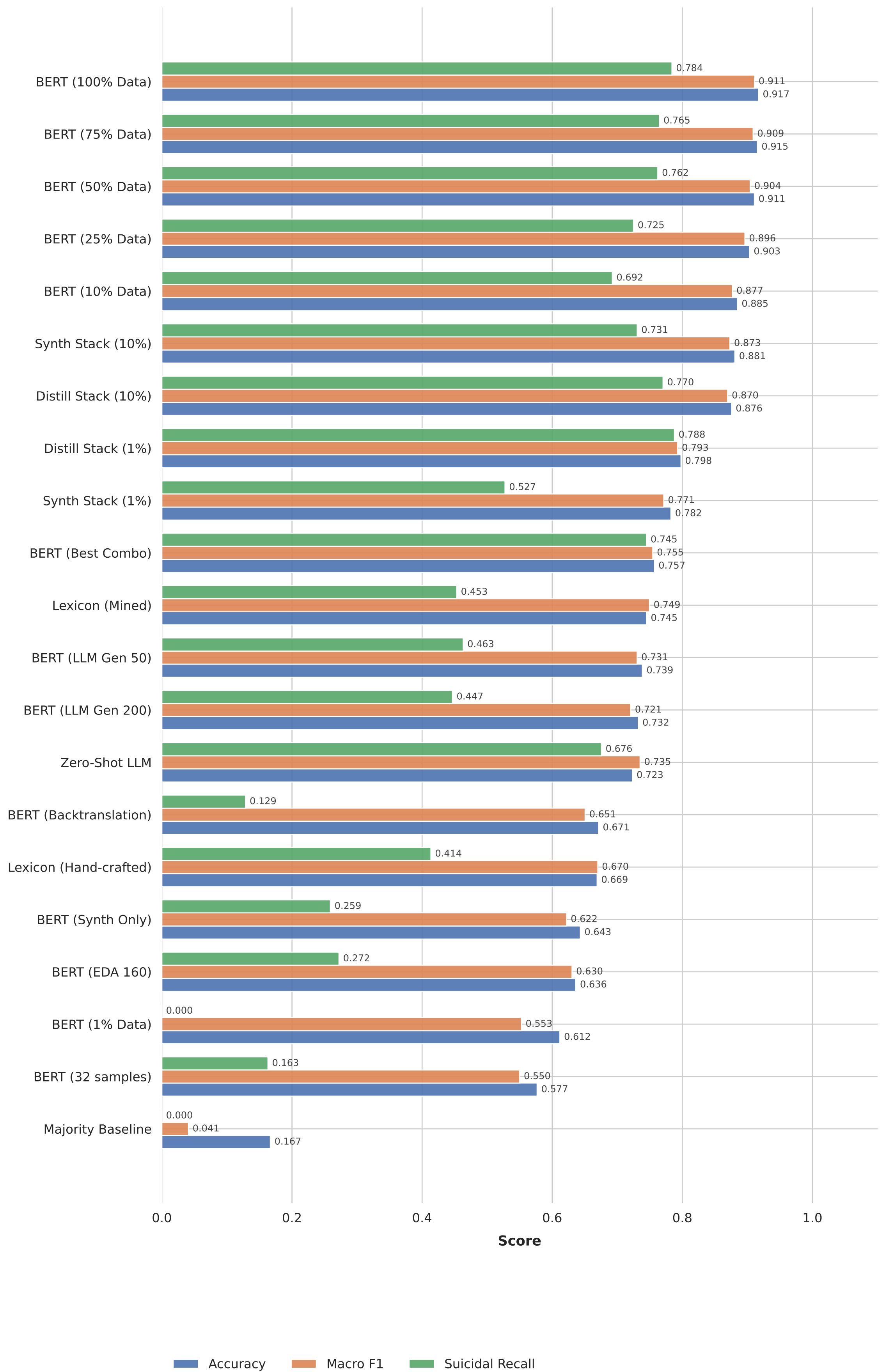
Combined Performance: Accuracy, Macro F1, and Suicidal Recall
