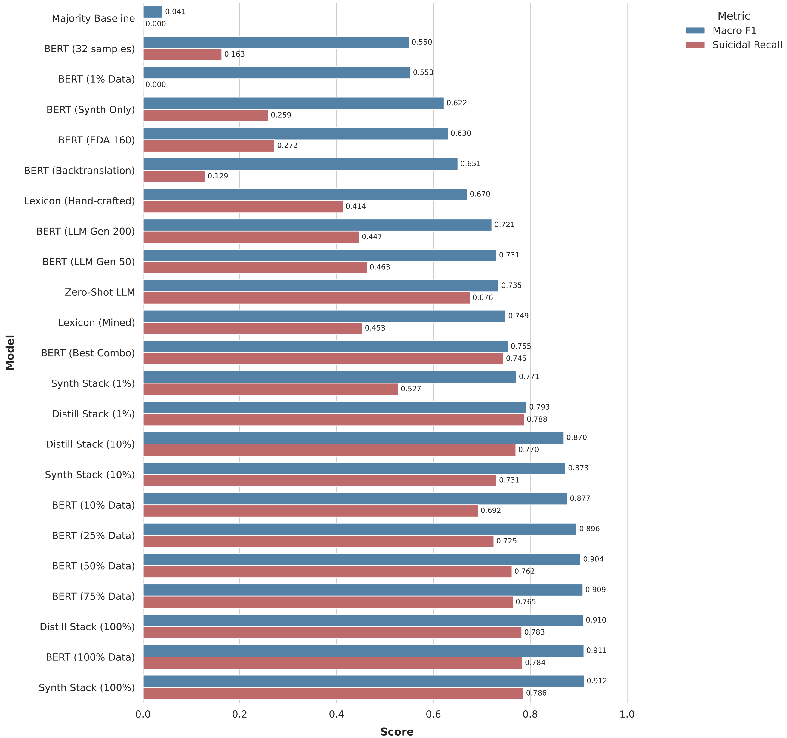
Model Performance: Macro F1 vs. Suicidal Recall
