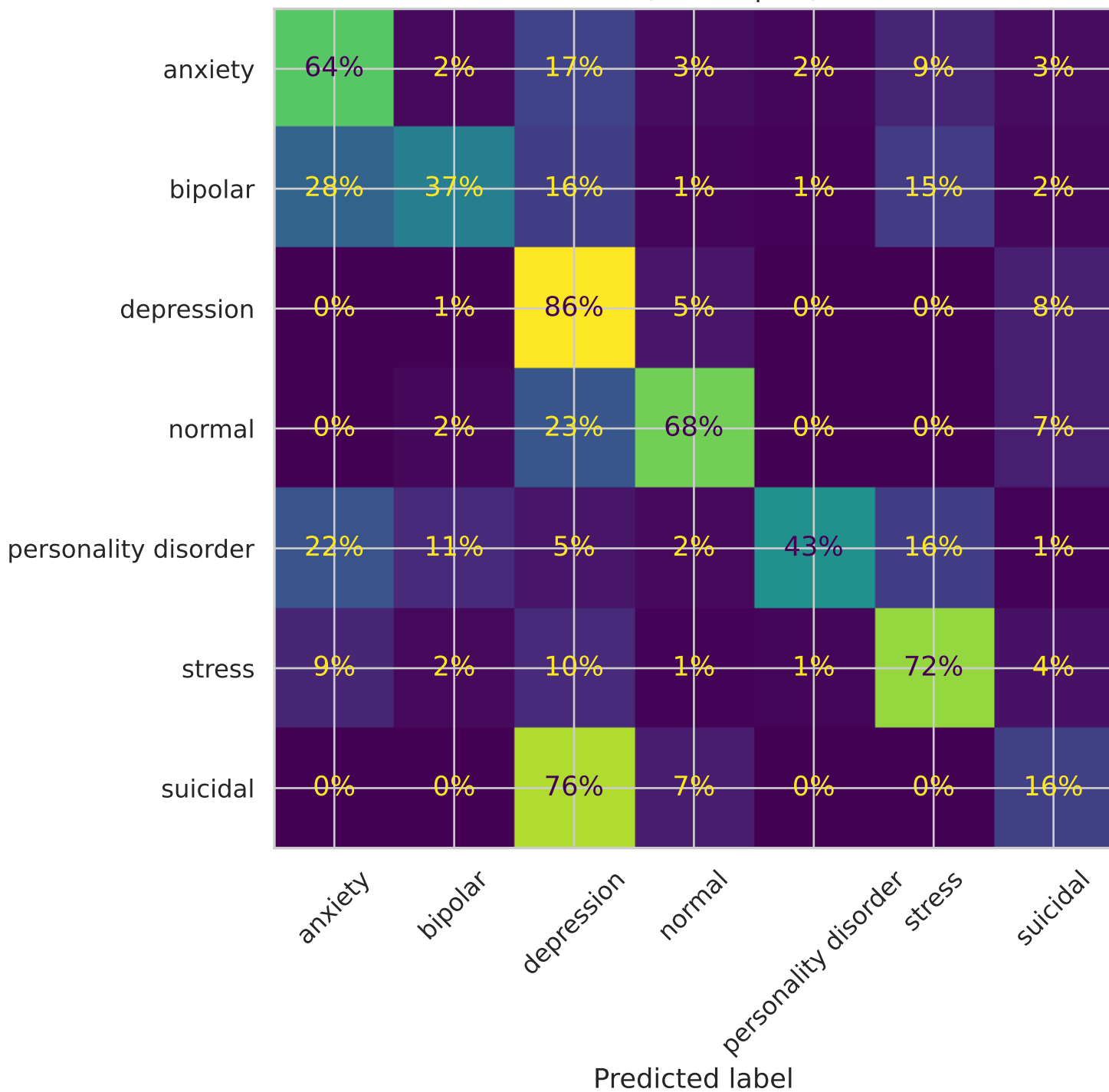
BERT (32 samples)
