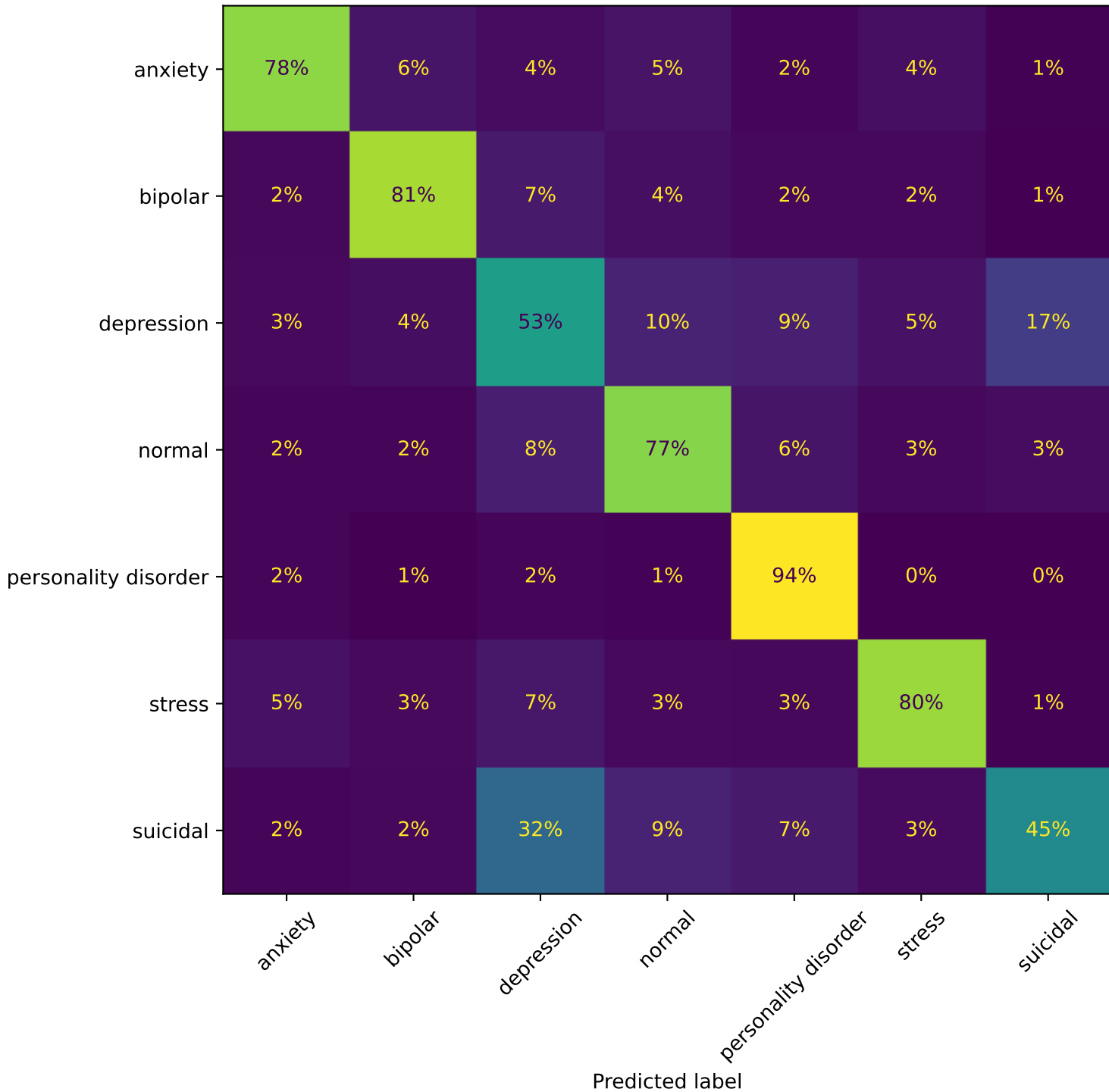
BERT + LLM-gen 200/class (32+1400) - Confusion Matrix (row-normalised)
