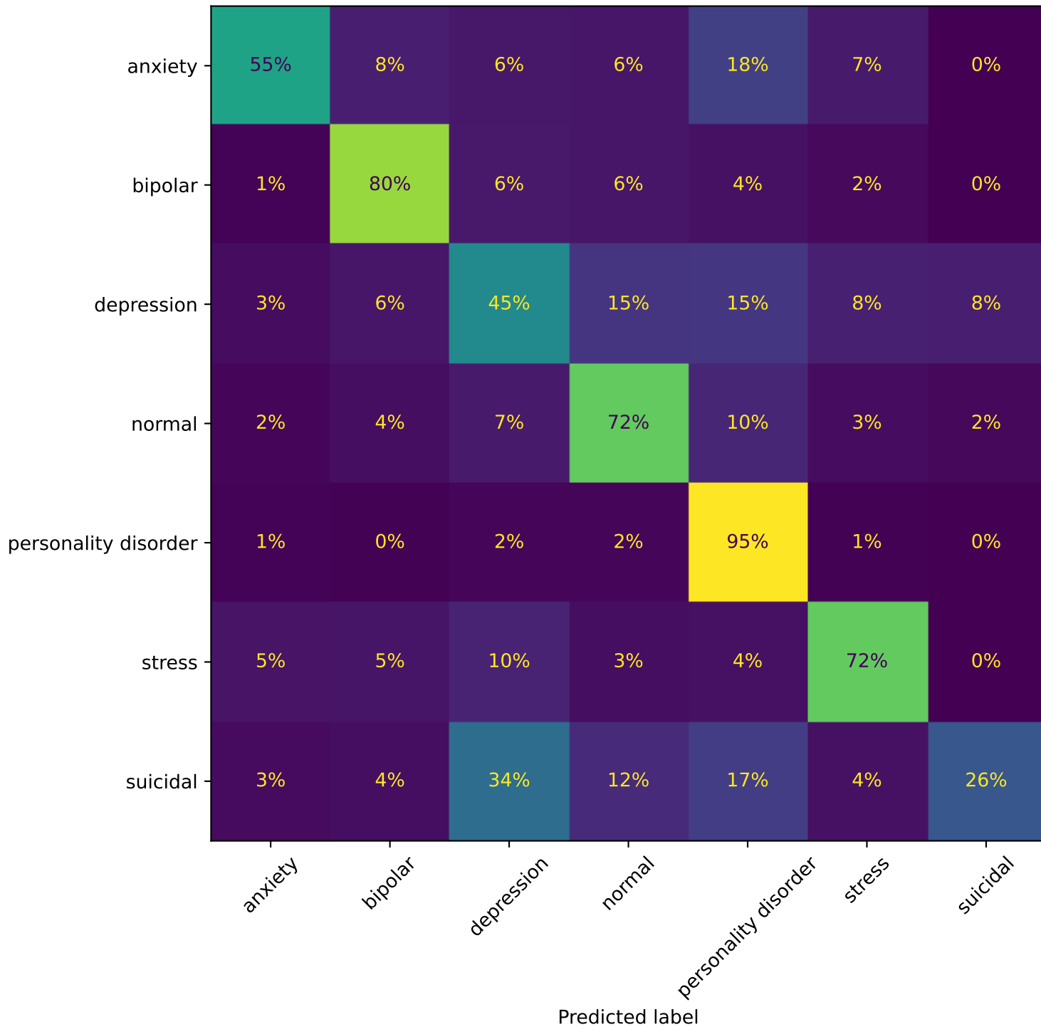
BERT synthetic-only (1400, no real labels) - Confusion Matrix (row-normalised)
