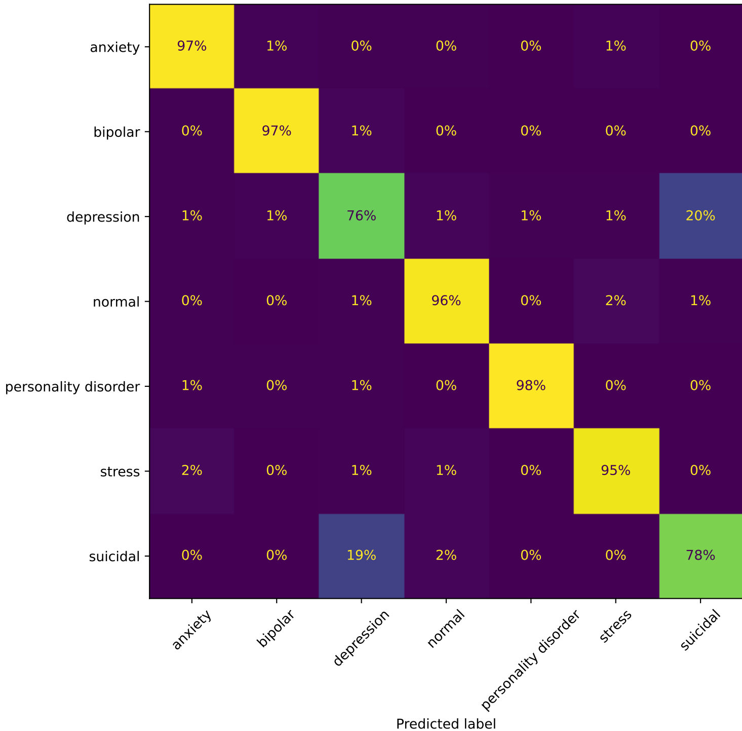
part3 bert pct100 - Confusion Matrix (row-normalised)
