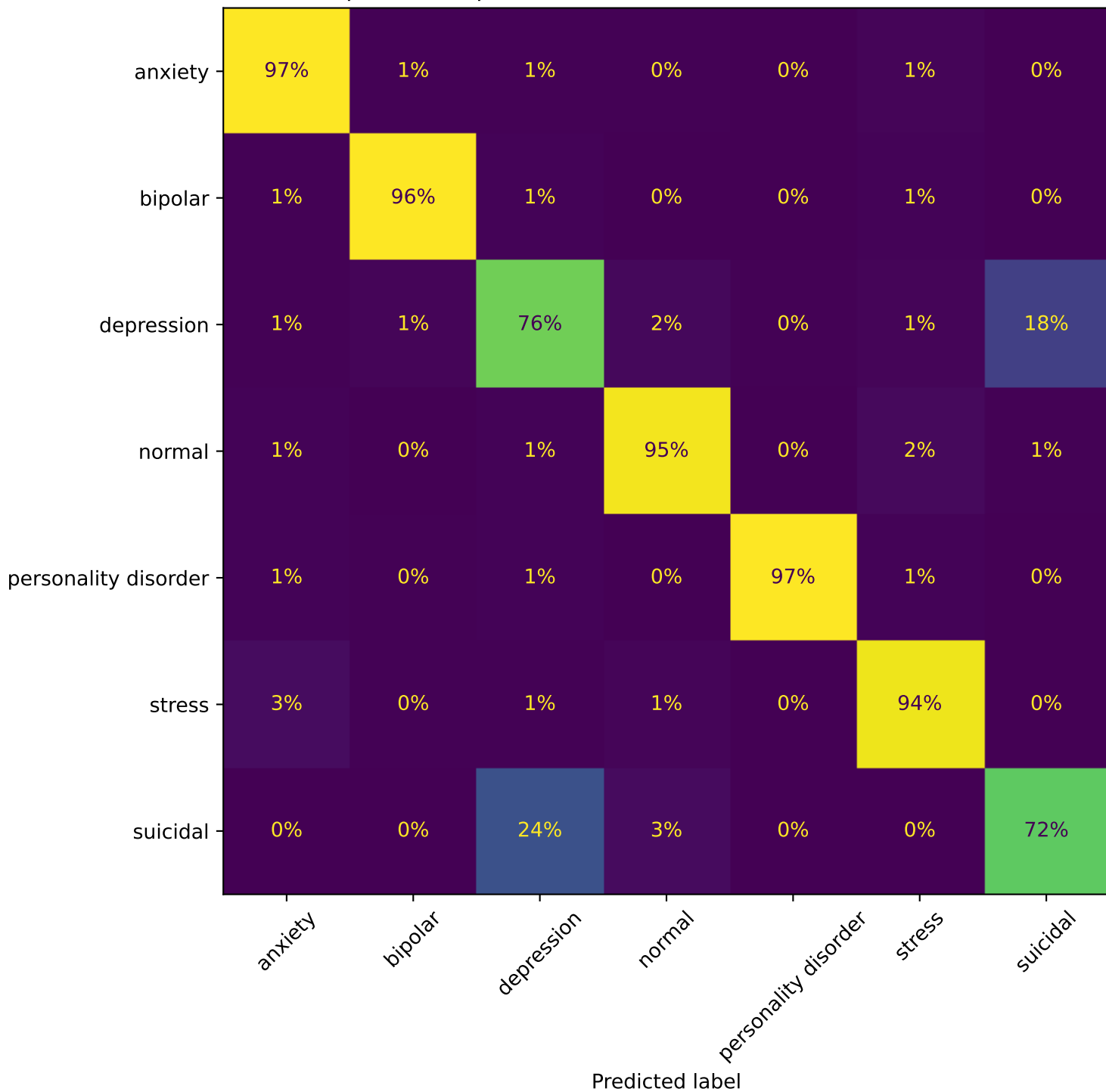
part3 bert pct25 - Confusion Matrix (row-normalised)
