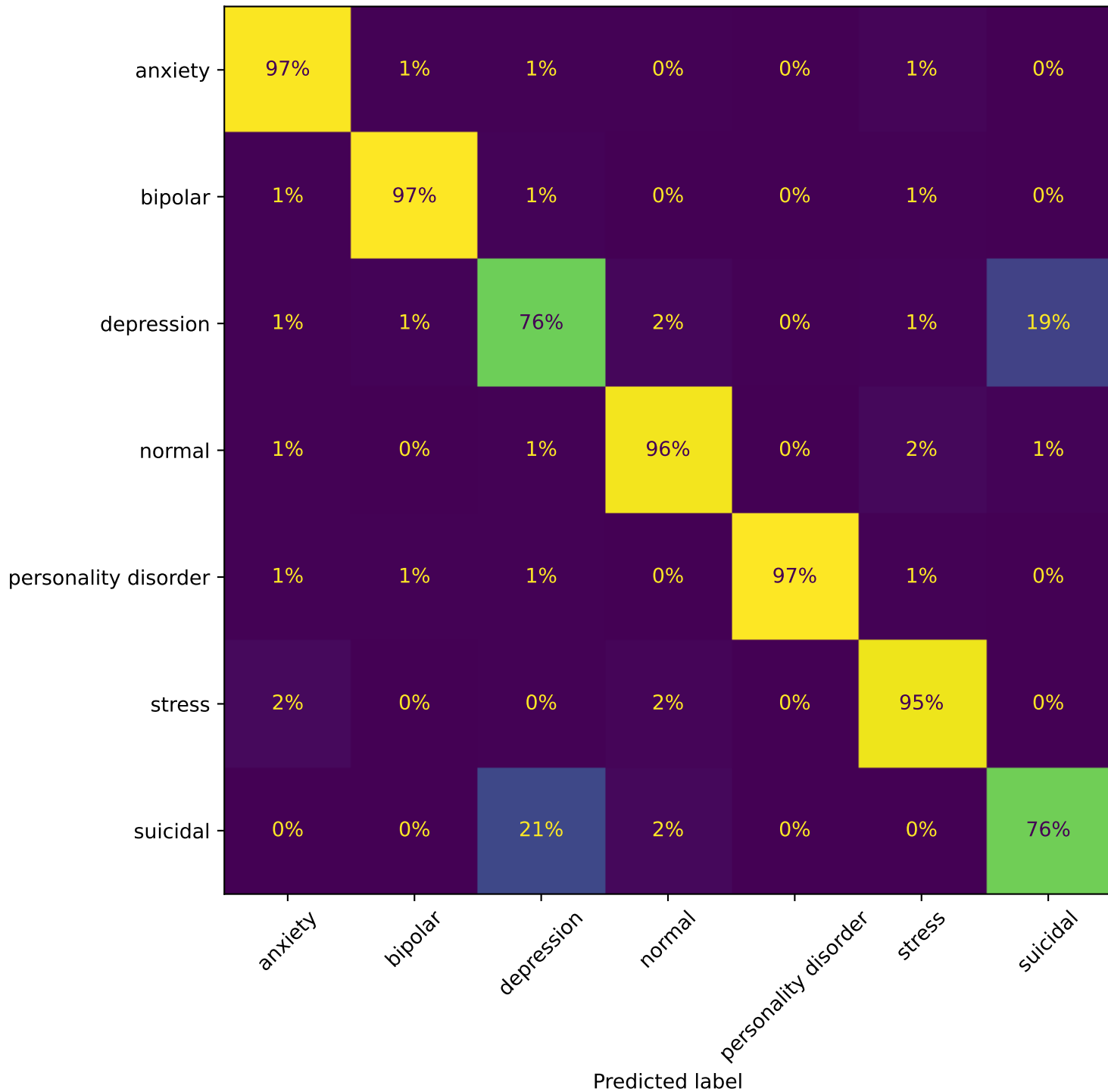
part3 bert pct50 - Confusion Matrix (row-normalised)
