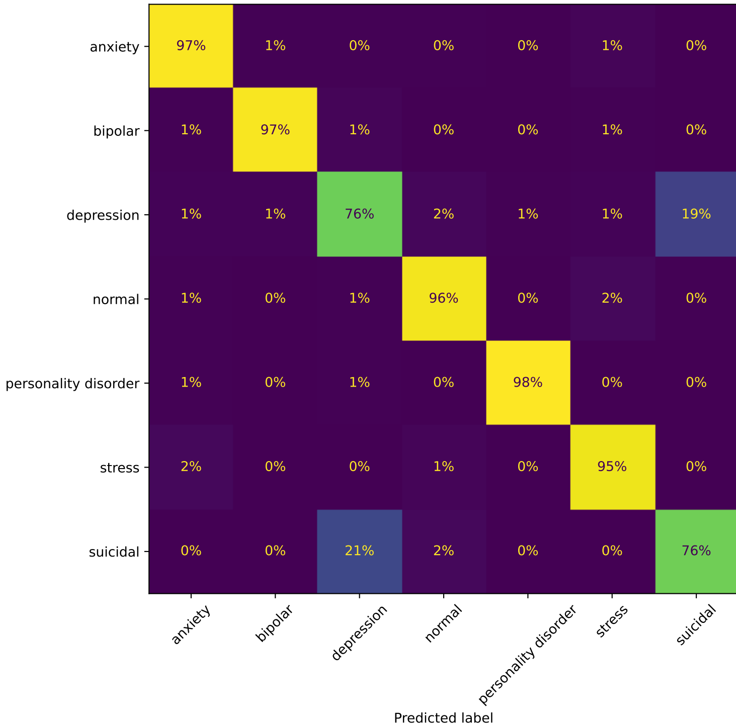
part3 bert pct75 - Confusion Matrix (row-normalised)
