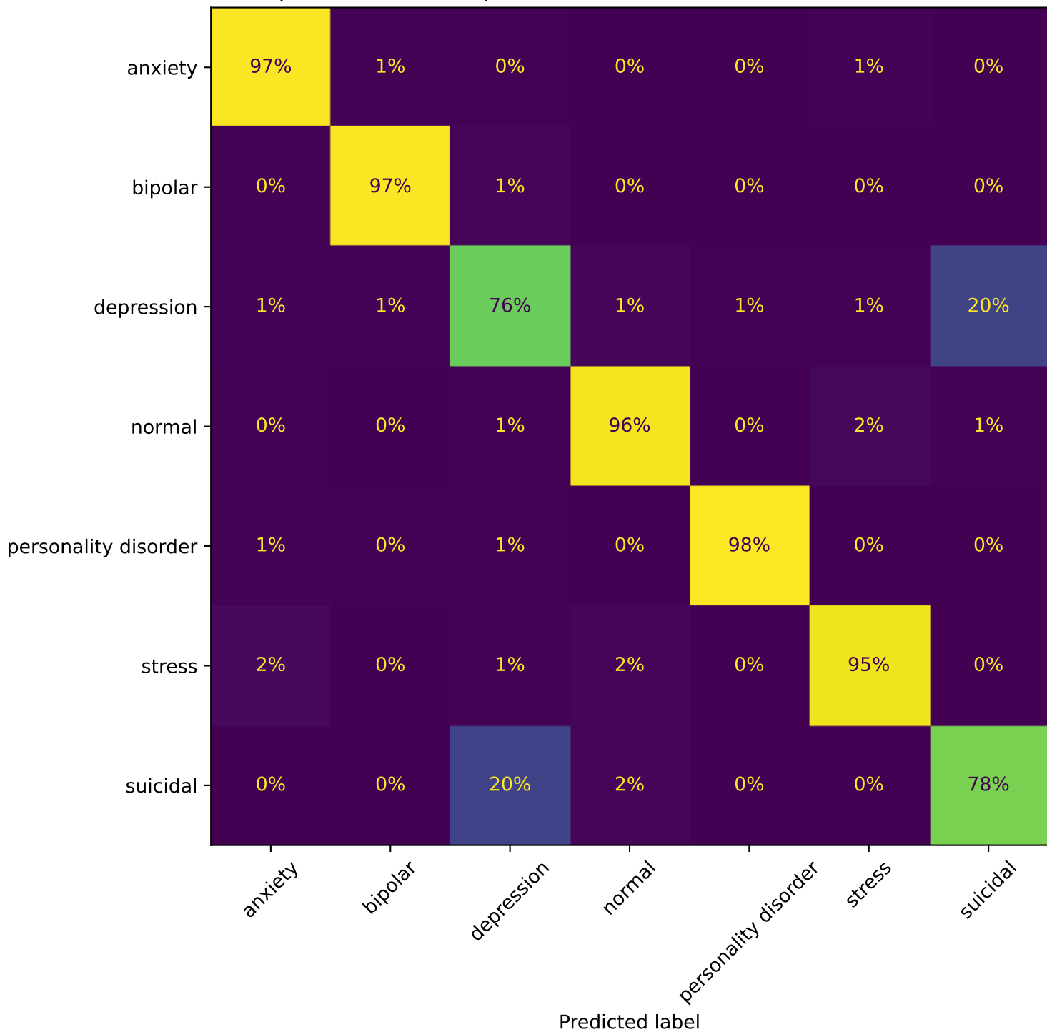
part3 distill stack pct100 - Confusion Matrix (row-normalised)
