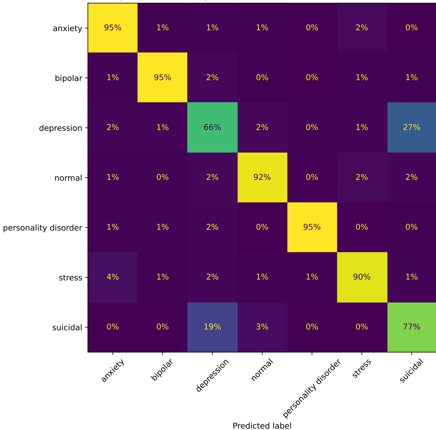
part3 distill stack pct10 - Confusion Matrix (row-normalised)
