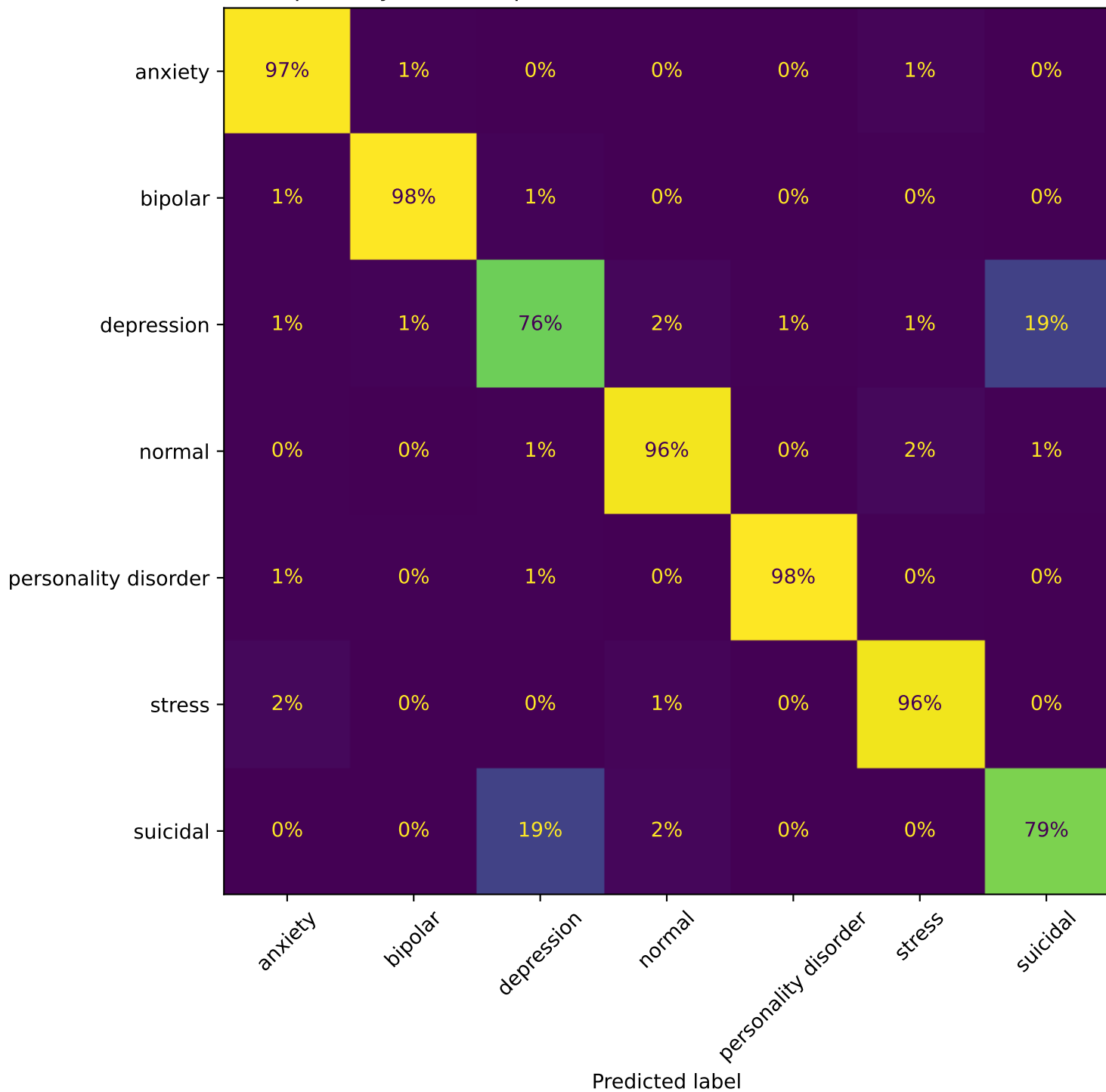
part3 synth stack pct100 - Confusion Matrix (row-normalised)
