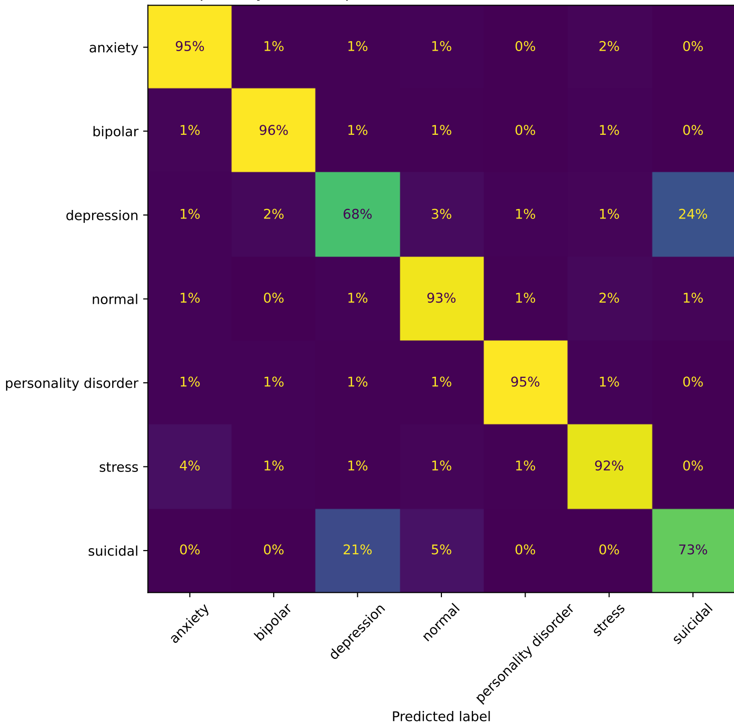
part3 synth stack pct10 - Confusion Matrix (row-normalised)
