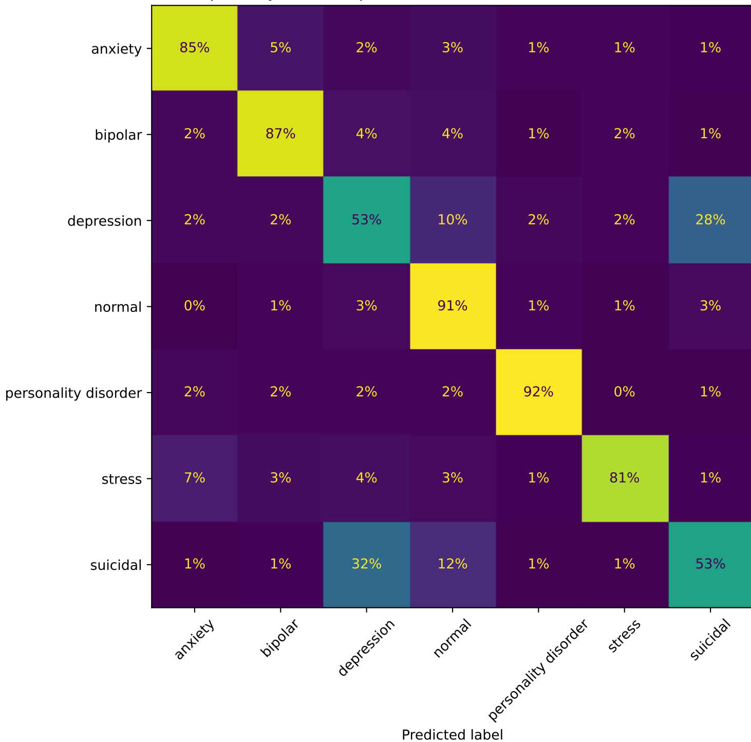
part3 synth stack pct1 - Confusion Matrix (row-normalised)
