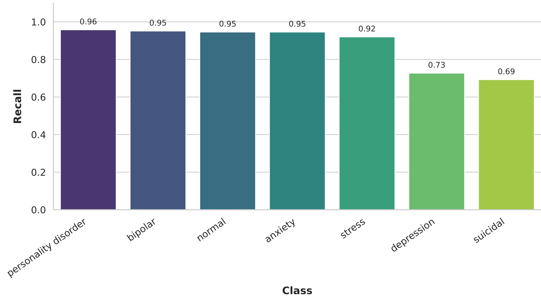
Per-Class Recall for BERT (10% Data)
