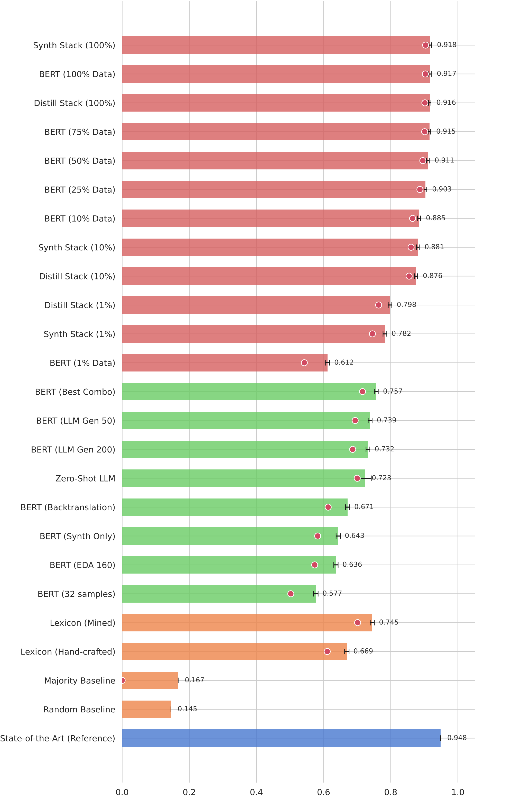
Results Ladder: Accuracy and Agreement on Frozen Test Set (Grouped by Part)
