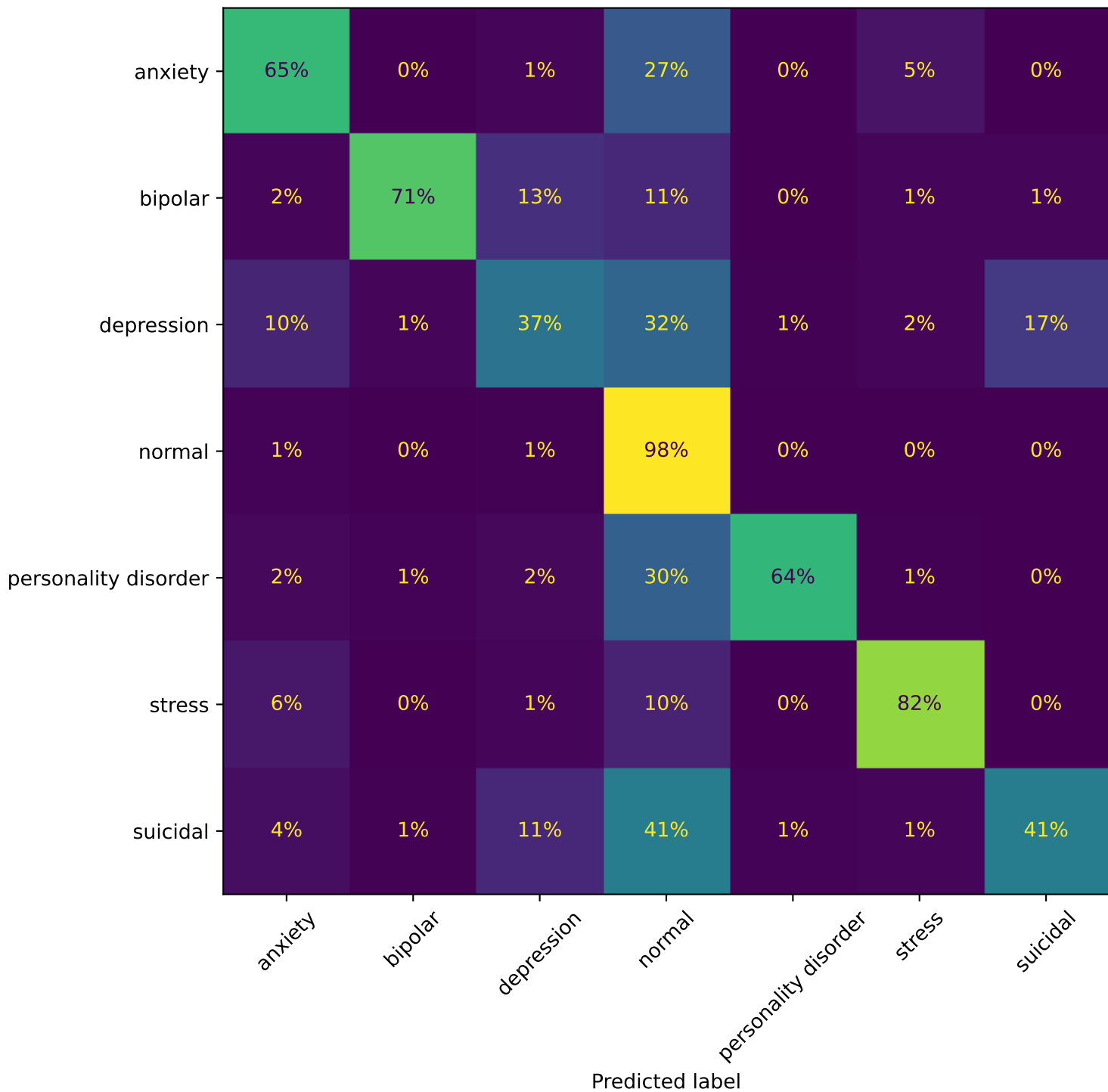
Rule-Based Classifier - Confusion Matrix (row-normalised)
