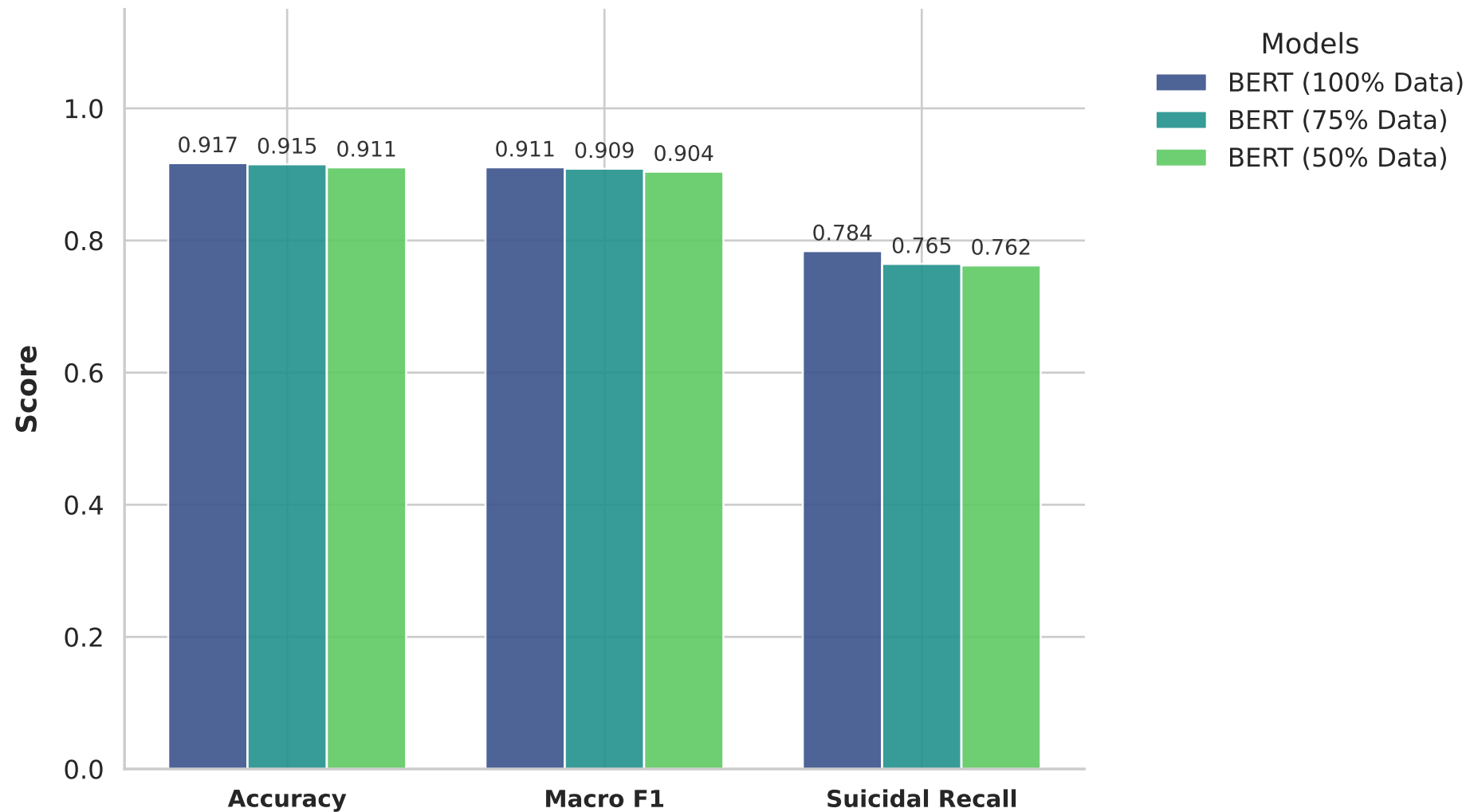
Top 3 Models Comparison: Key Metrics
