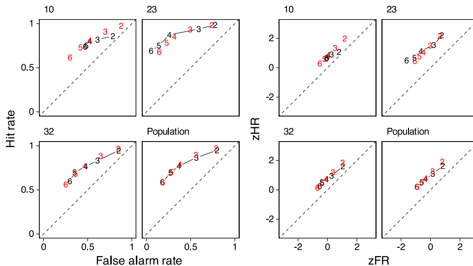
Figure A1.1. Receiver operating characteristic plots in the proportion (left) and z-score scales (right) for three participants and the population. Black symbols and lines are coordinates calculated from data, red symbols are model-predicted rates.
