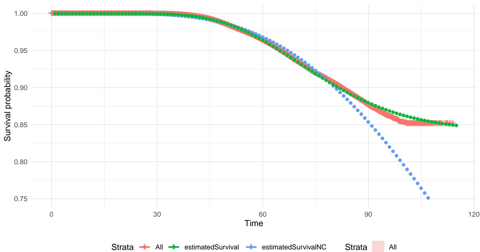
Multivariate Gamma on All Subjects
