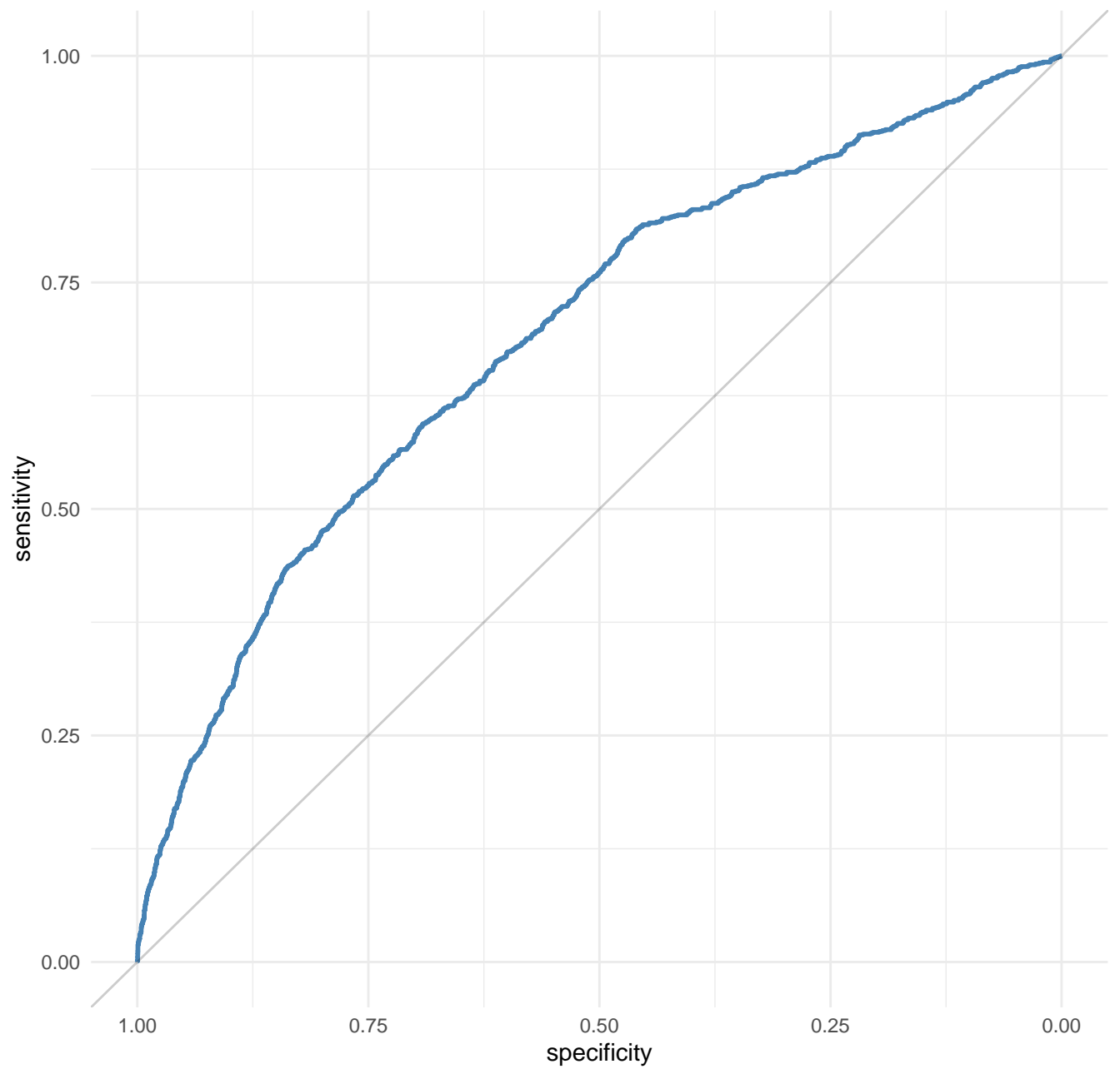
ROC curve (AUC = 0.6917)
