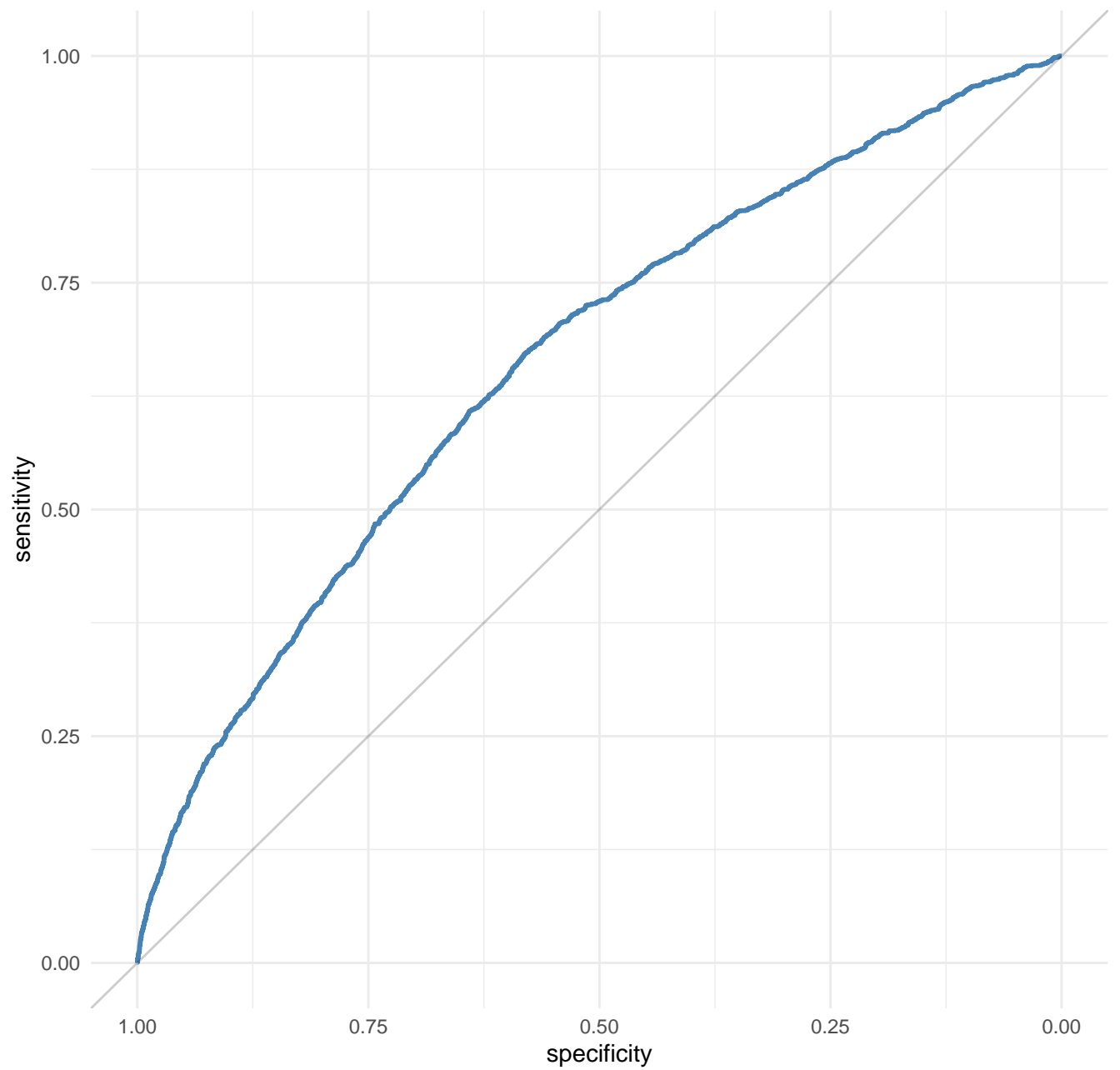
ROC curve (AUC = 0.6627)
