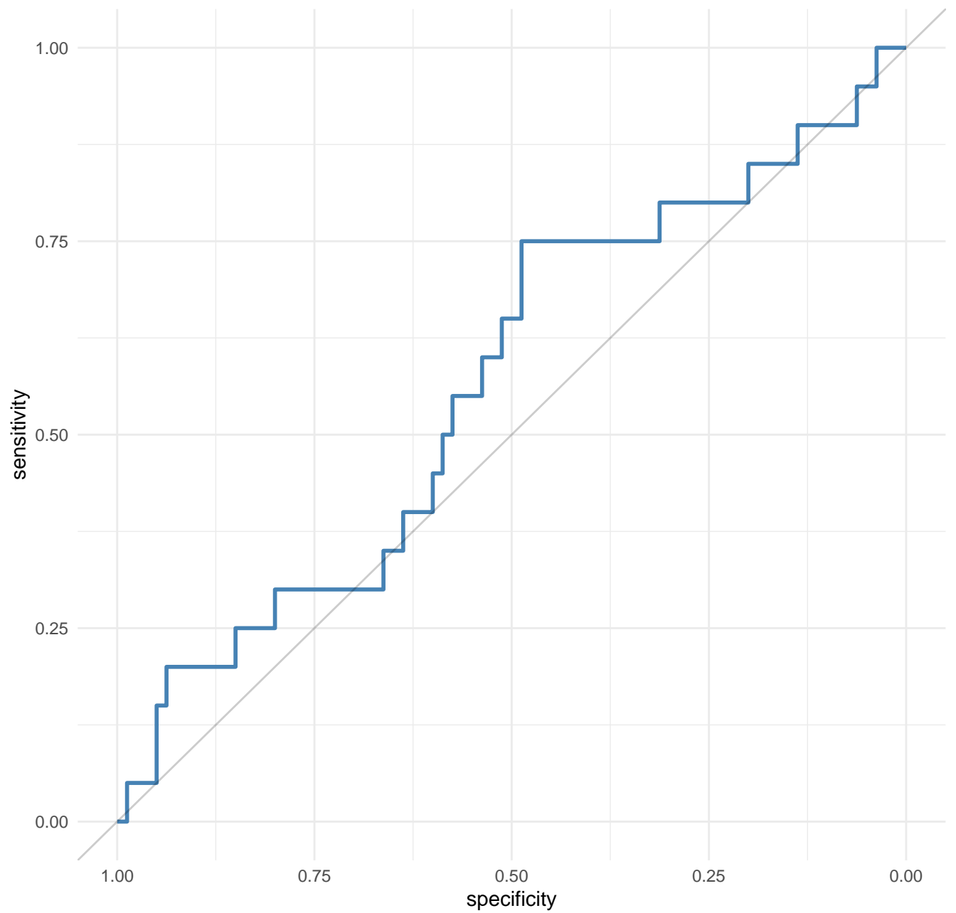
ROC curve (AUC = 0.5656)
