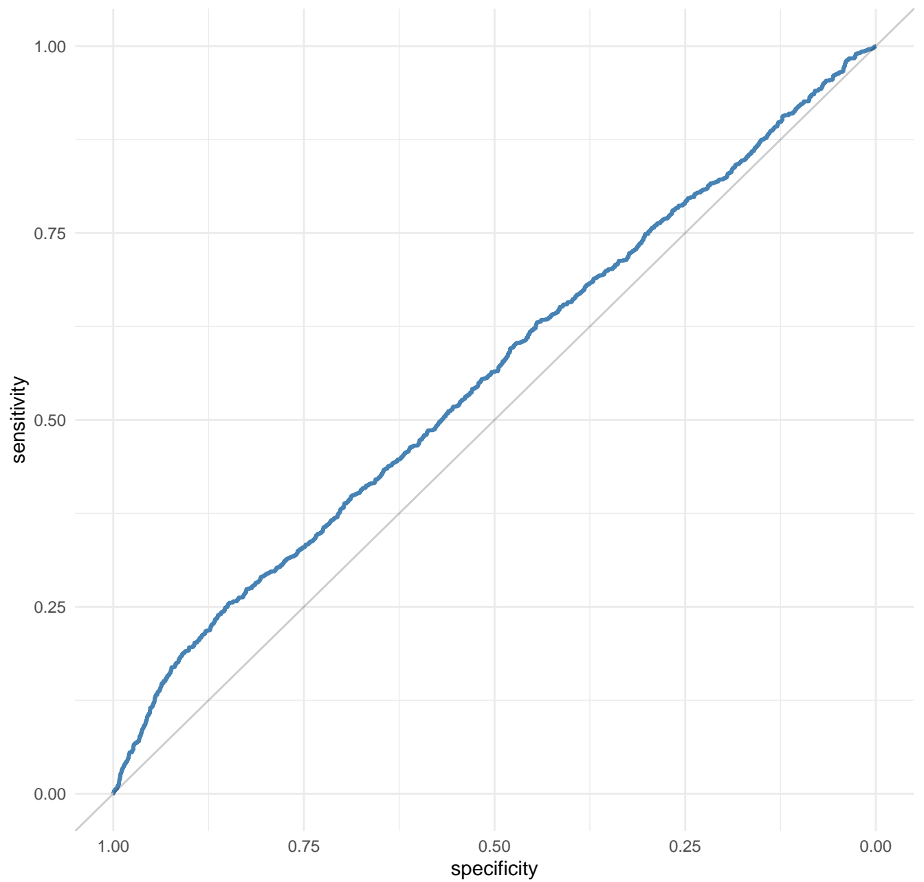
ROC curve (AUC = 0.5577)
