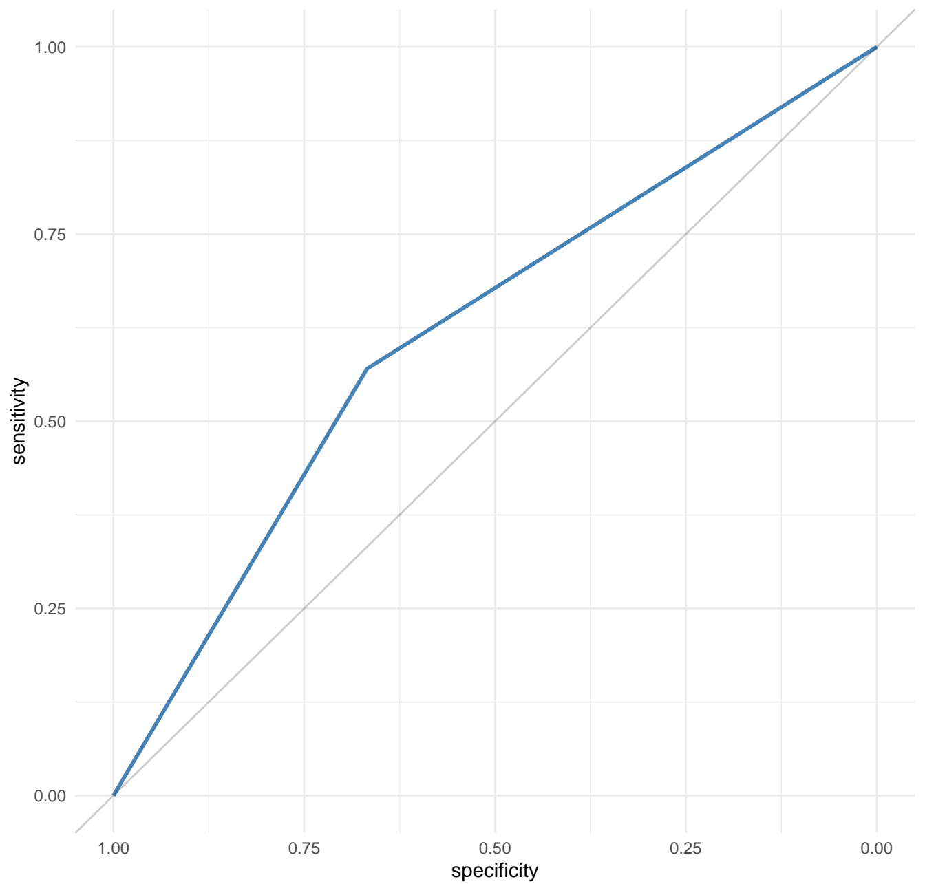
ROC curve (AUC = 0.6189)
