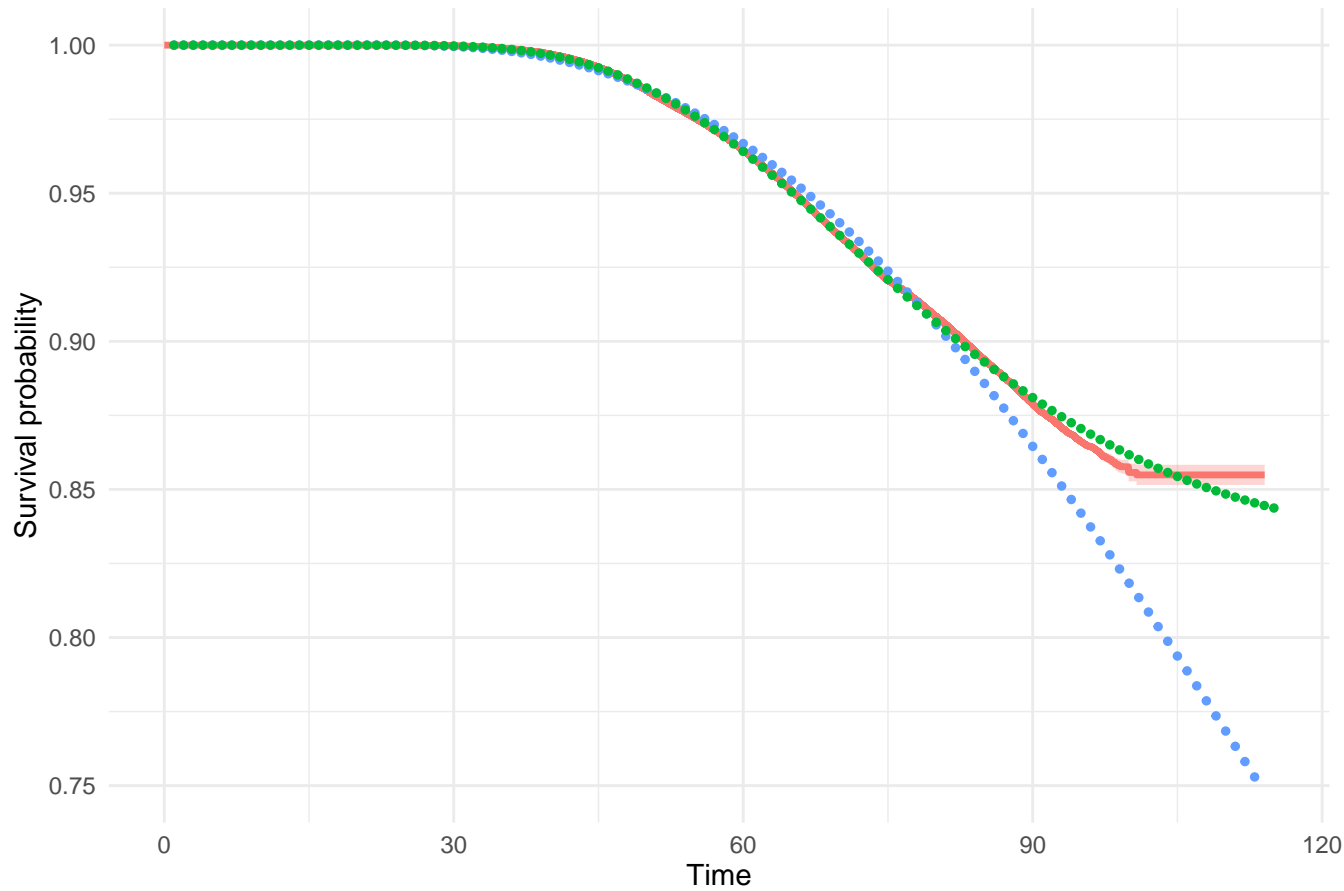
Multivariate 3-parameters Gamma for all subjects
