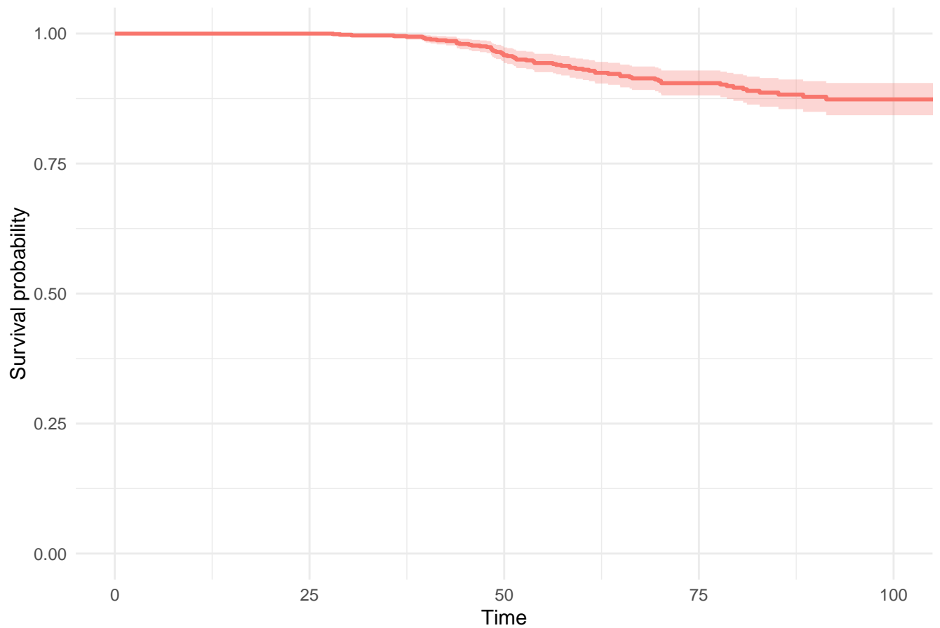
Kaplan–Meier on Main Subjects for 3-parameters Gamma
