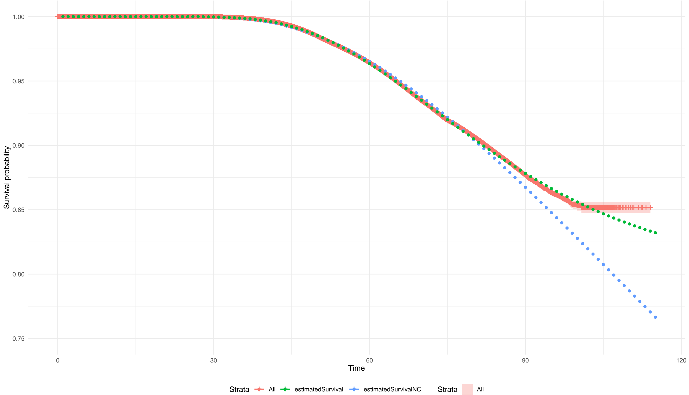
Multivariate 3-pars LogNormal on All
