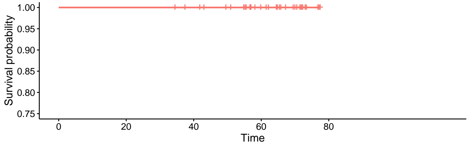
Kaplan–Meier on Eight Sister
