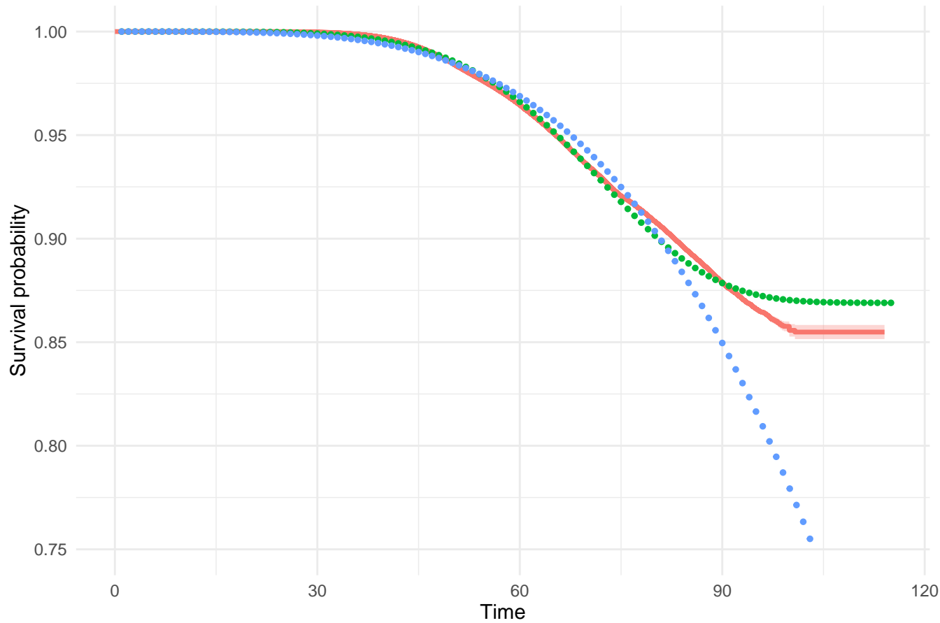
Multivariate Weibull for all subjects
