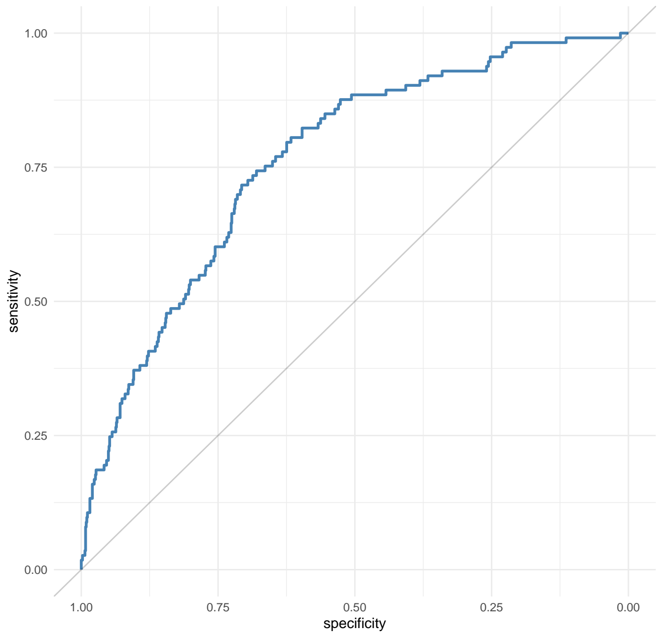
ROC curve (AUC = 0.7621)
