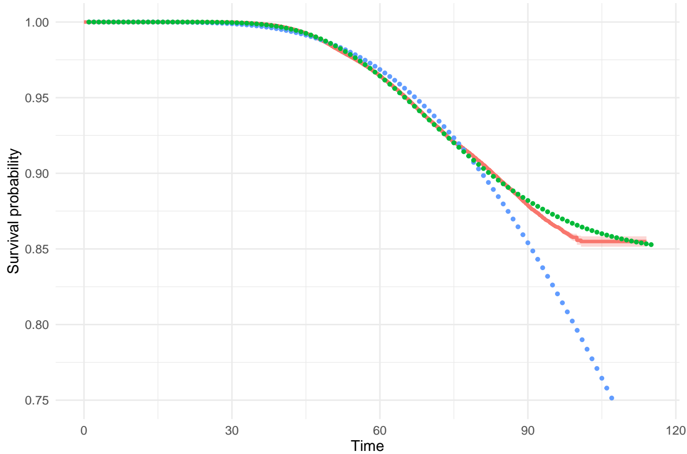
Multivariate Gamma for all subjects
