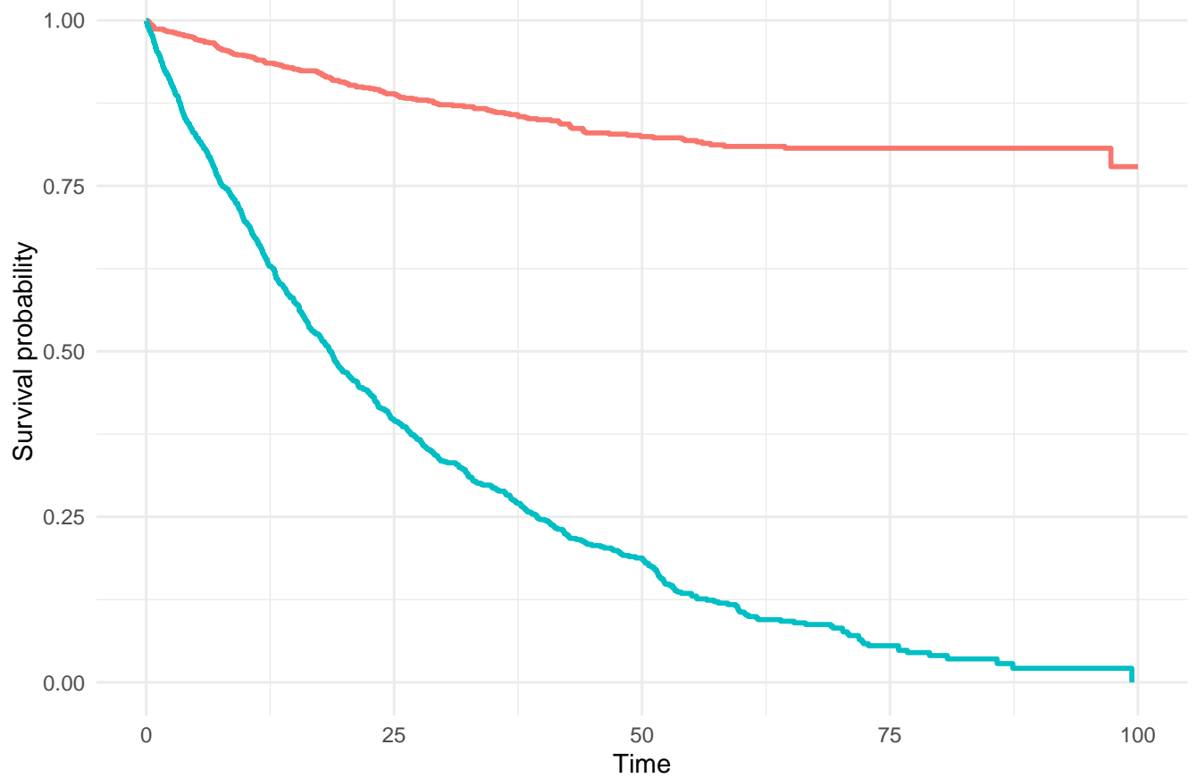
Traditional vs. Cure Rate survival function
