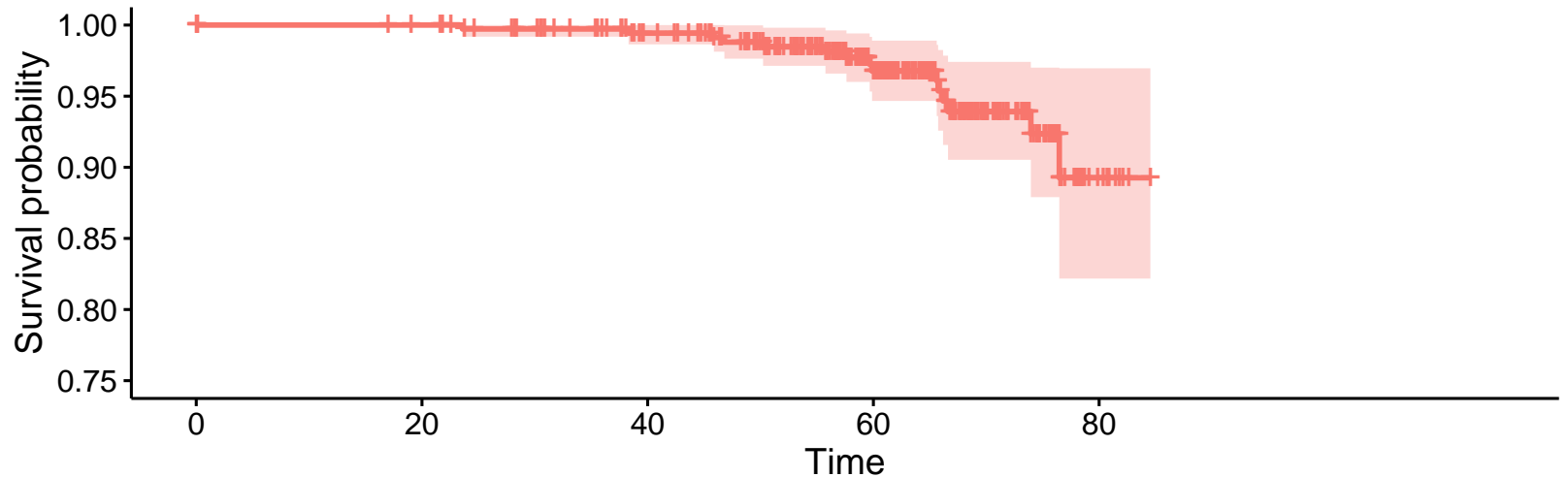
Kaplan–Meier on Sixth Sister
