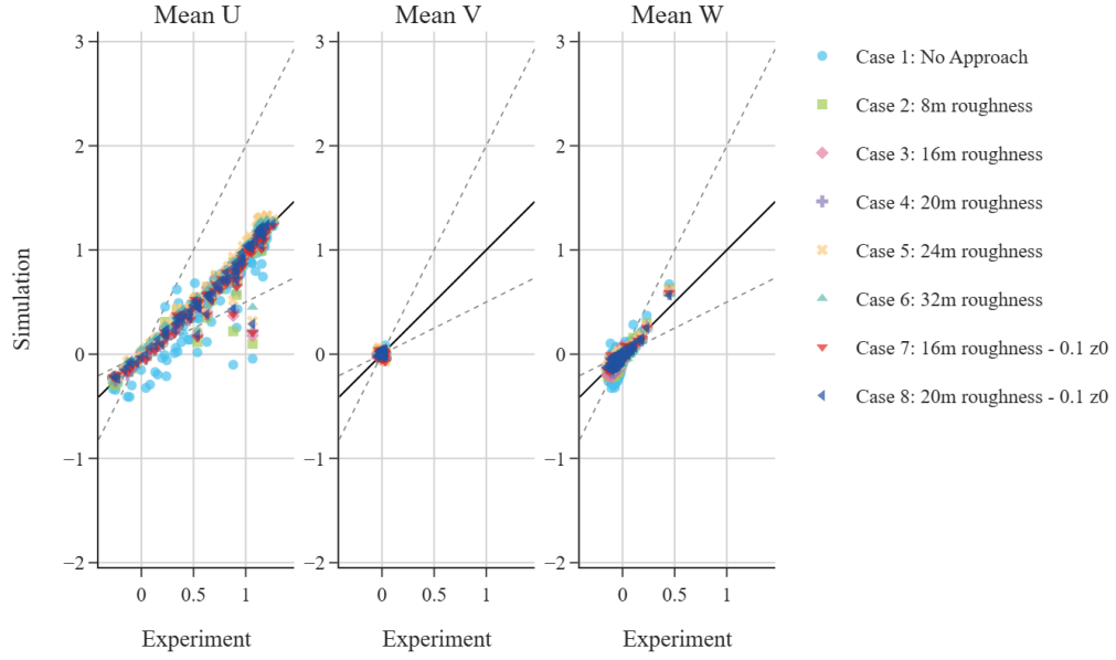
Figure 14: Scatter plot comparison of normalized mean velocity components (\bar{u}, \bar{v}, \bar{w}) against AIJ experimental data across all cases. Solid lines represent the 1:1 correlation, while dashed lines indicate the FAC2 boundaries.
