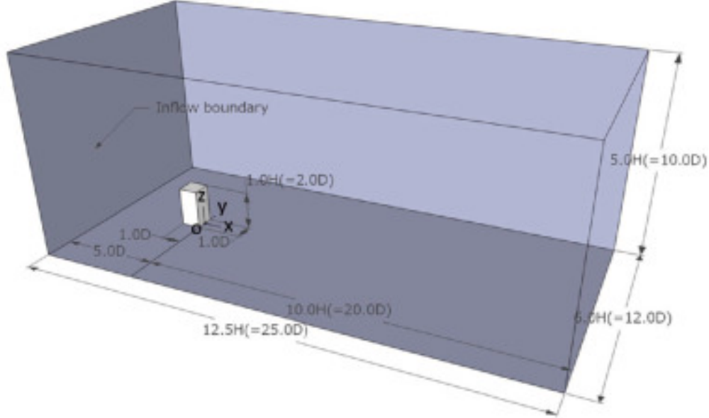
Figure 3: Numerical domain configuration and measurement locations for the LES validation study (adapted from Okaze et al., 2021).
