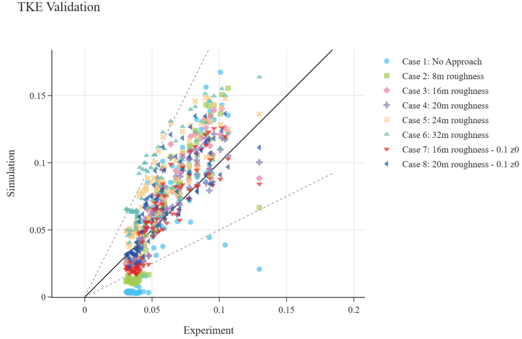
Figure 15: Correlation of predicted vs. observed Turbulent Kinetic Energy ( k ), highlighting the impact of the refined z_0 and roughness configurations on energy modeling accuracy.
