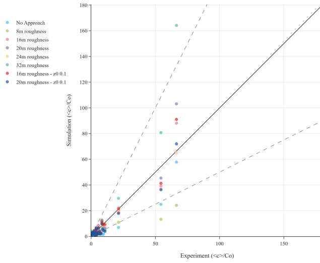
Figure 17: Scatter plot comparison of normalized concentration ( C_{norm} ) results against AIJ experimental data. The solid line indicates the 1:1 ideal correlation, while the dashed lines represent the FAC2 boundaries.
