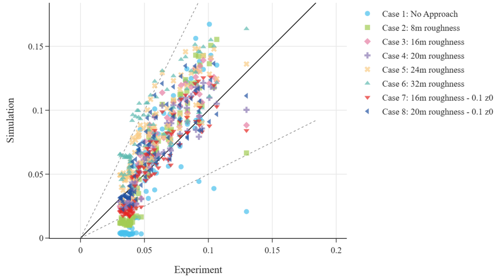
Figure 16: Correlation of predicted vs. observed Turbulent Kinetic Energy ( k ), highlighting the impact of the refined z_0 and roughness configurations on energy modeling accuracy.
