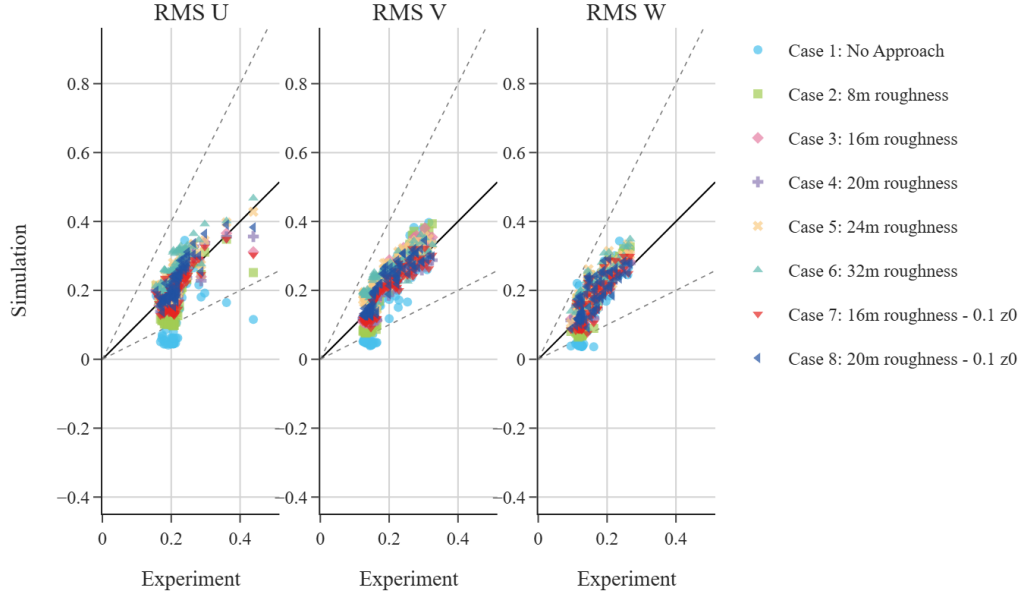
Figure 15: Validation scatter plot for RMS velocity fluctuations ( u_{rms}, v_{rms}, w_{rms} ), demonstrating the solver's ability to capture turbulence intensity across the domain.
