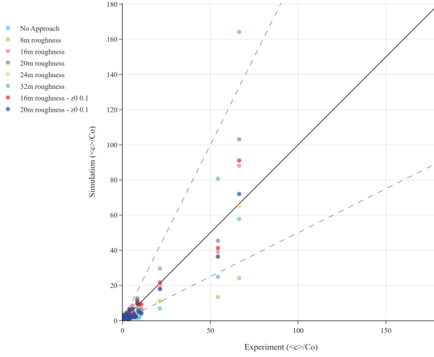
Figure 18: Scatter plot comparison of normalized concentration ( C_{norm} ) results against AIJ experimental data. The solid line indicates the 1:1 ideal correlation, while the dashed lines represent the FAC2 boundaries.
