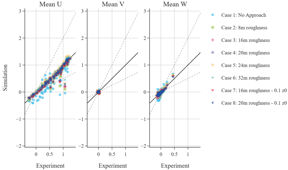
Figure 14: Scatter plot comparison of normalized mean velocity components ( \bar{u}, \bar{v}, \bar{w} ) against AIJ experimental data across all cases. Solid lines represent the 1:1 correlation, while dashed lines indicate the FAC2 boundaries.
