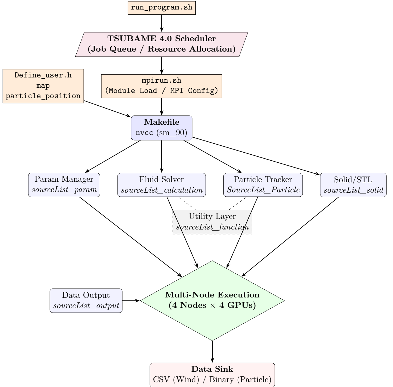
Figure 4: System architecture of the LBM simulation framework executed using the TSUBAME 4.0 Supercomputer
