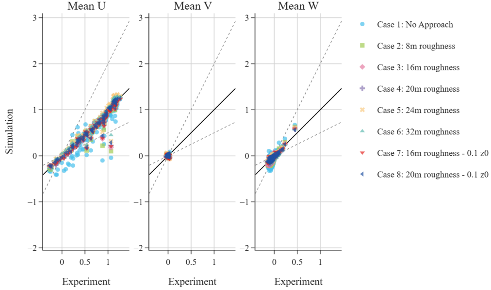
Figure 14: Scatter plot comparison of normalized mean velocity components ( \bar{u} , \bar{v} , \bar{w} ) against AIJ experimental data across all cases. Solid lines represent the 1:1 correlation, while dashed lines indicate the FAC2 boundaries.
