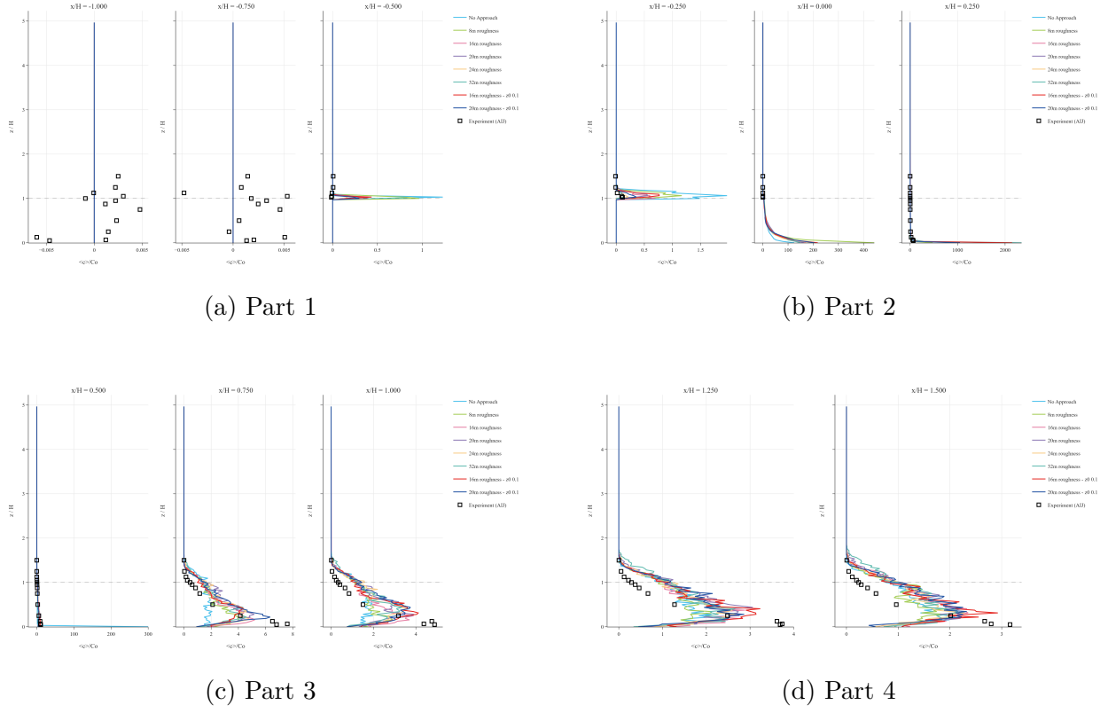
Figure 17: Normalized concentration ( C_{norm} ) profiles across 11 AIJ measurement locations, divided into (a) Part 1, (b) Part 2, (c) Part 3, and (d) Part 4.
