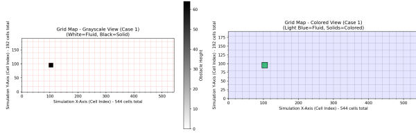
(a) Case 1: No approach flow
