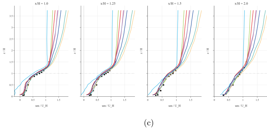
Figure 7: Normalized mean streamwise velocity ( \bar{u}/U_H ) profiles at (a) Windward locations ( x/H = -1.0 to -0.25 ), (b) Near Wake locations ( x/H = 0.0 to 0.75 ), and (c) Far Wake locations ( x/H = 1.0 to 2.0 ).
