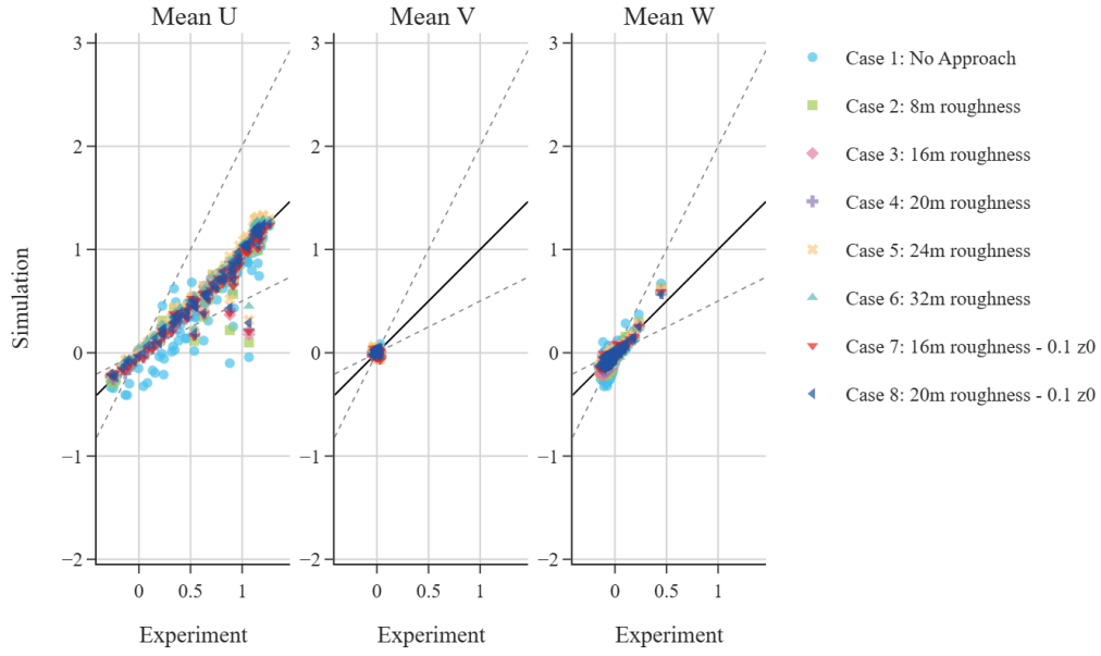
Figure 14: Scatter plot comparison of normalized mean velocity components (\bar{u}, \bar{v}, \bar{w}) against AIJ experimental data across all cases. Solid lines represent the 1:1 correlation, while dashed lines indicate the FAC2 boundaries.
