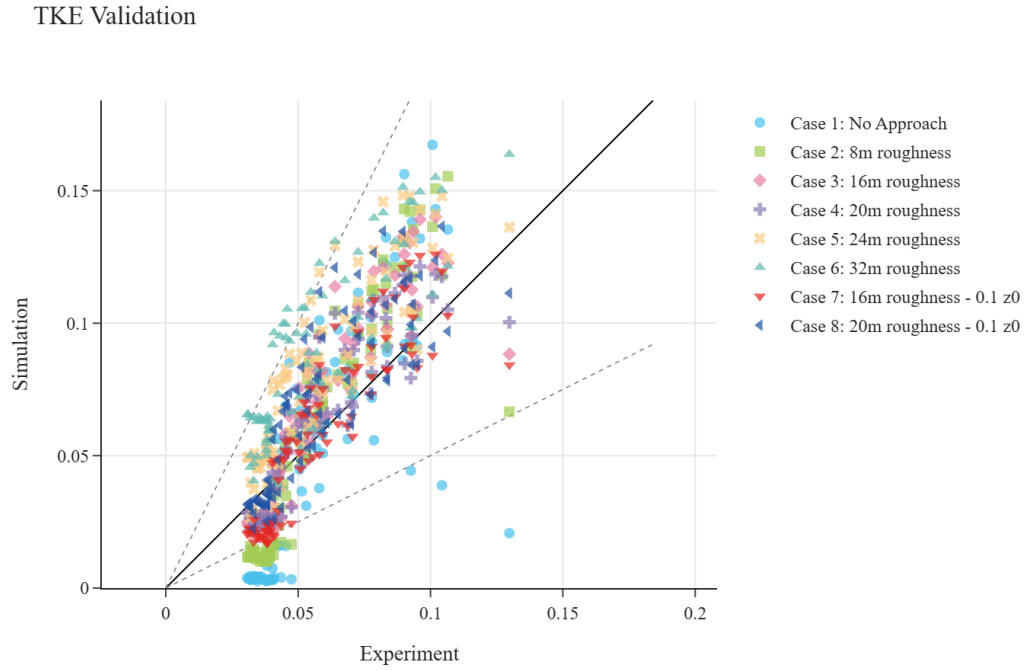
Figure 16: Correlation of predicted vs. observed Turbulent Kinetic Energy ( k ), highlighting the impact of the refined z_0 and roughness configurations on energy modeling accuracy.
