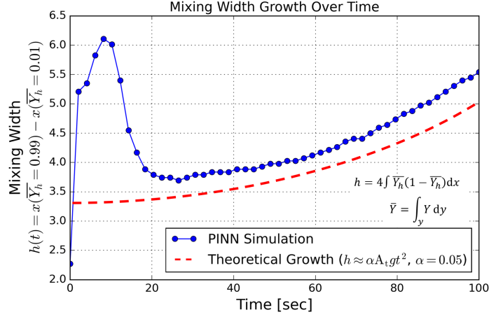
Figure 3: Mixing width h(t) predicted by the PINN compared to theoretical quadratic growth ( h \sim t^2 ).
