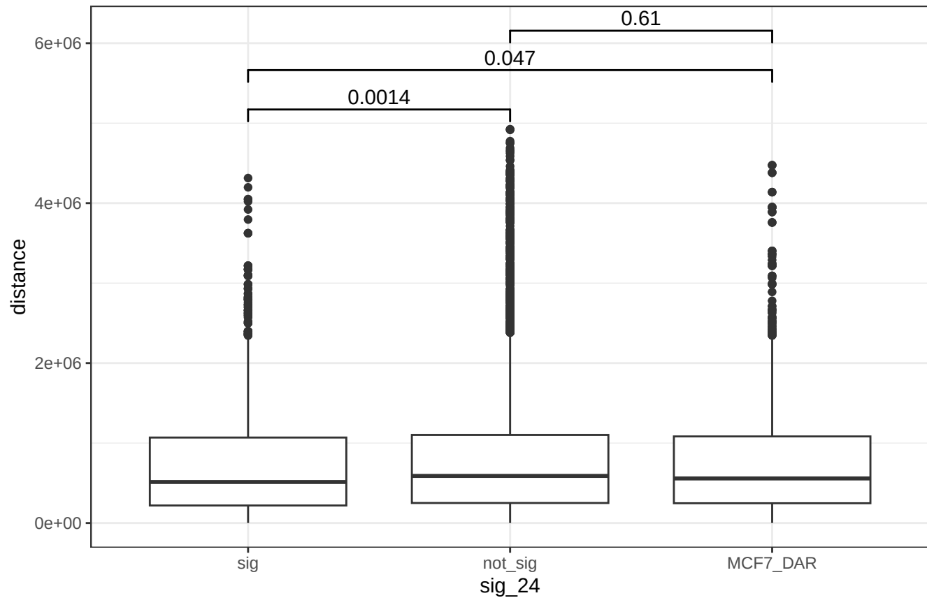
MTX 24 hour distances of DAR-SNP pairs and non-DAR-SNP pairs with MCF7 DARs
