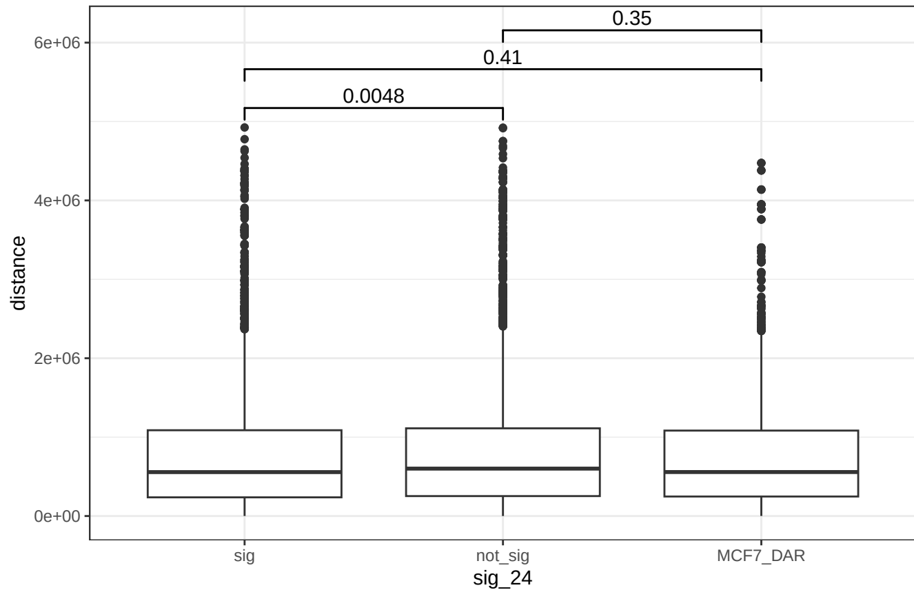
DNR 24 hour distances of DAR-SNP pairs and non-DAR-SNP pairs with MCF7 DARs
