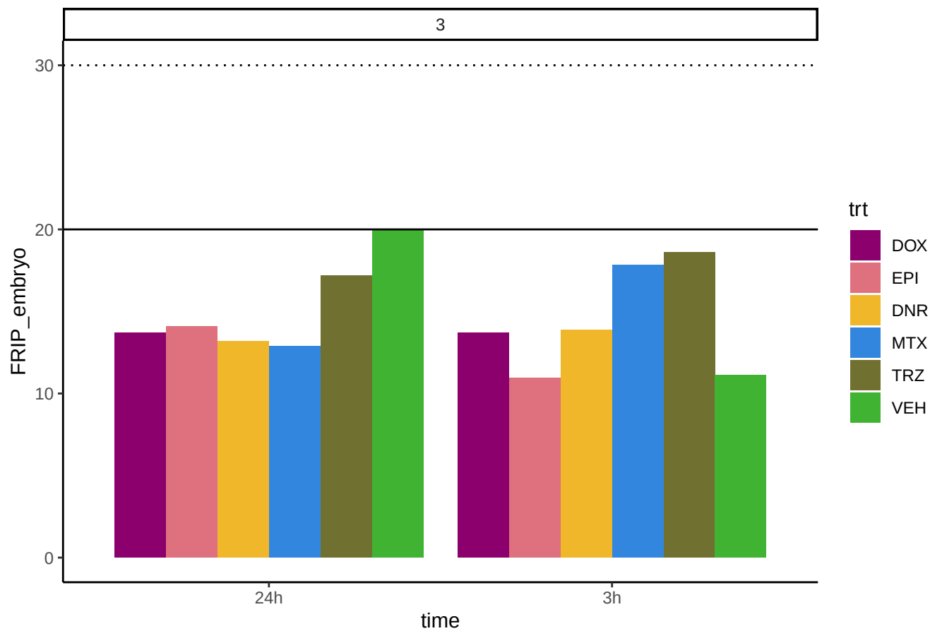
FRiP Score across Ind_B using embryonic heart DNase peaks
