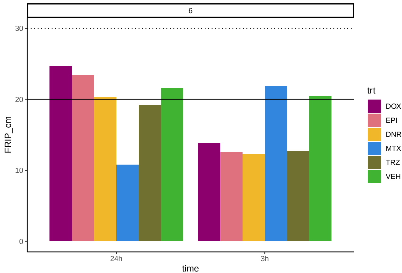
FRiP Score across Ind_C using cardiomyocyte DNase peaks
