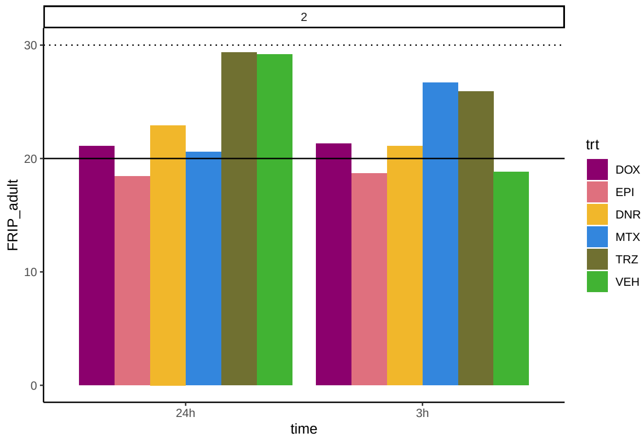
FRiP Score across IndA using adult heart DNase peaks
