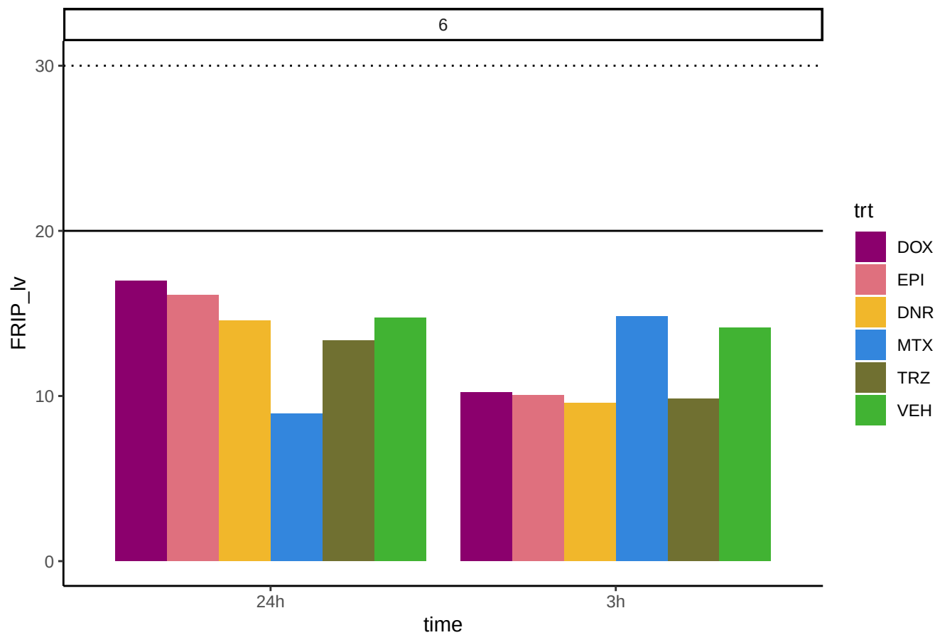
FRiP Score across Ind_C using left ventricle DNase peaks
