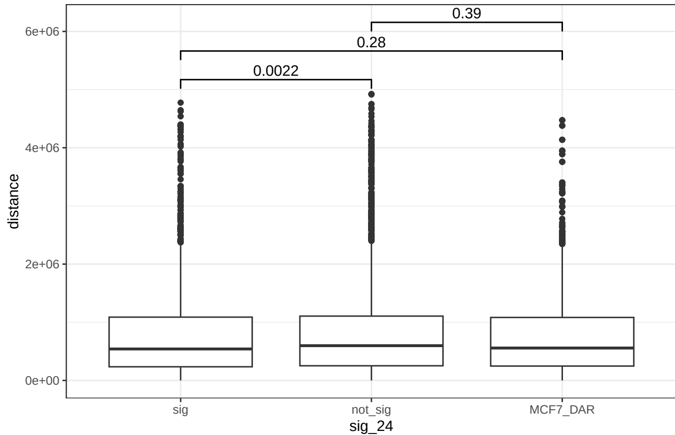
DOX 24 hour distances of DAR-SNP pairs and non-DAR-SNP pairs with MCF7 DARs
