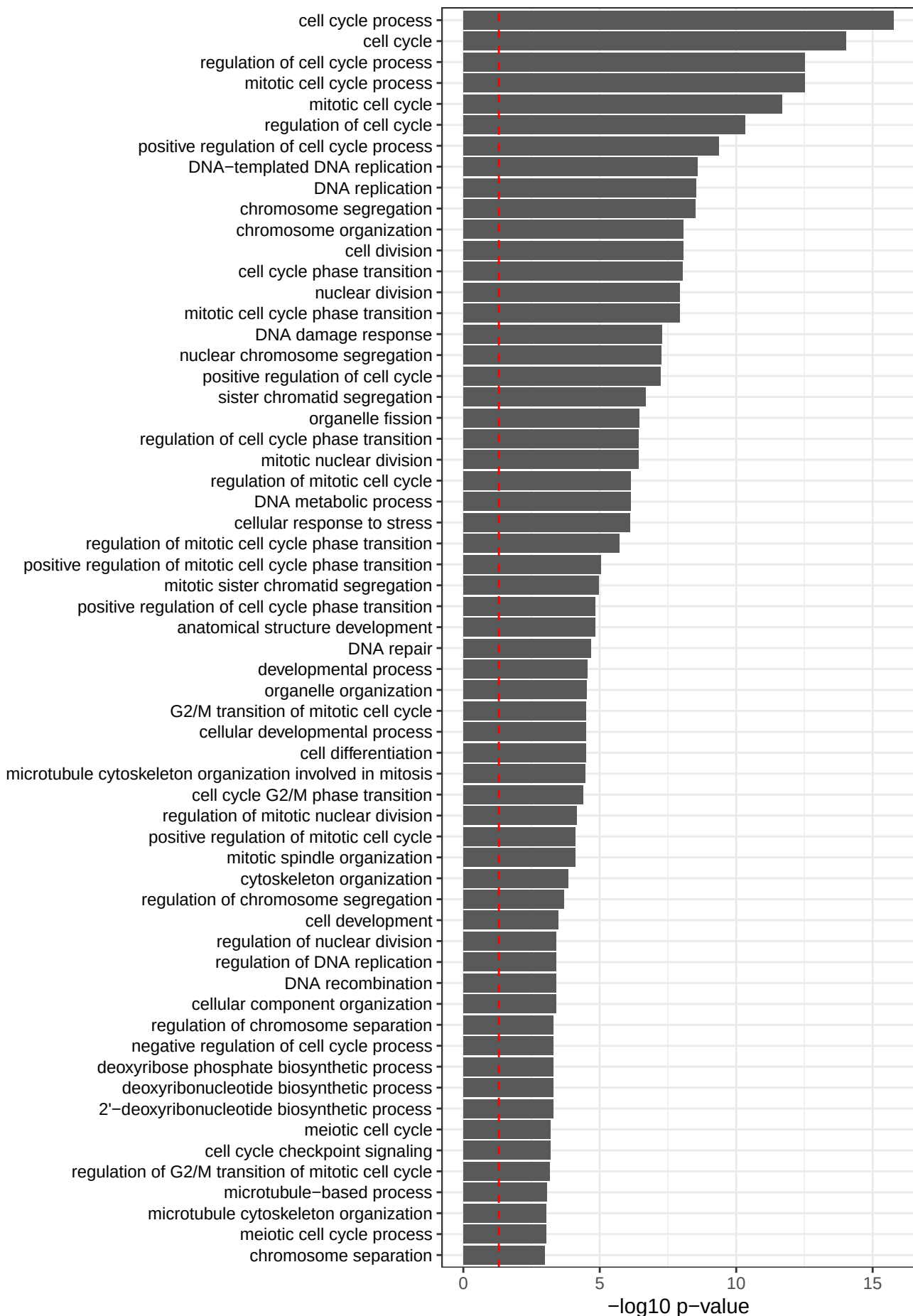
24 hour MTX_DAR_DEG pairs (within 2kb of
