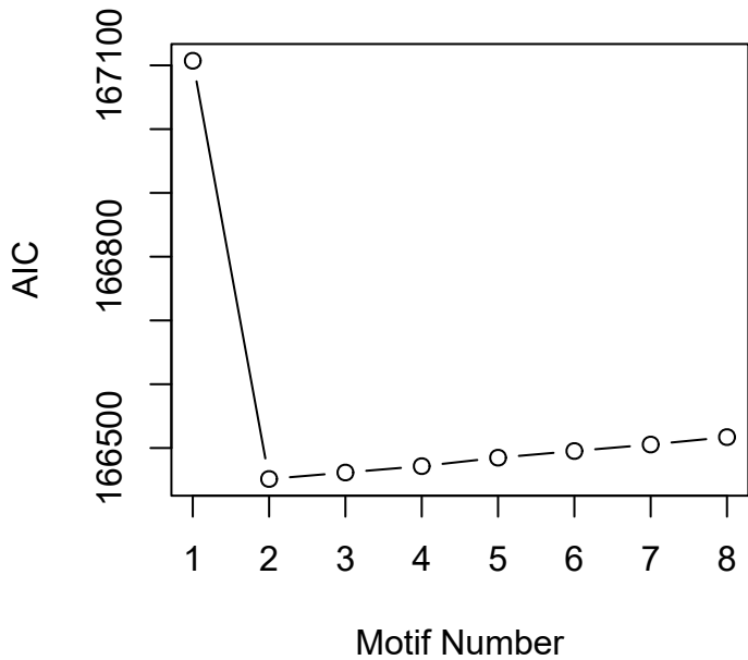
AIC
