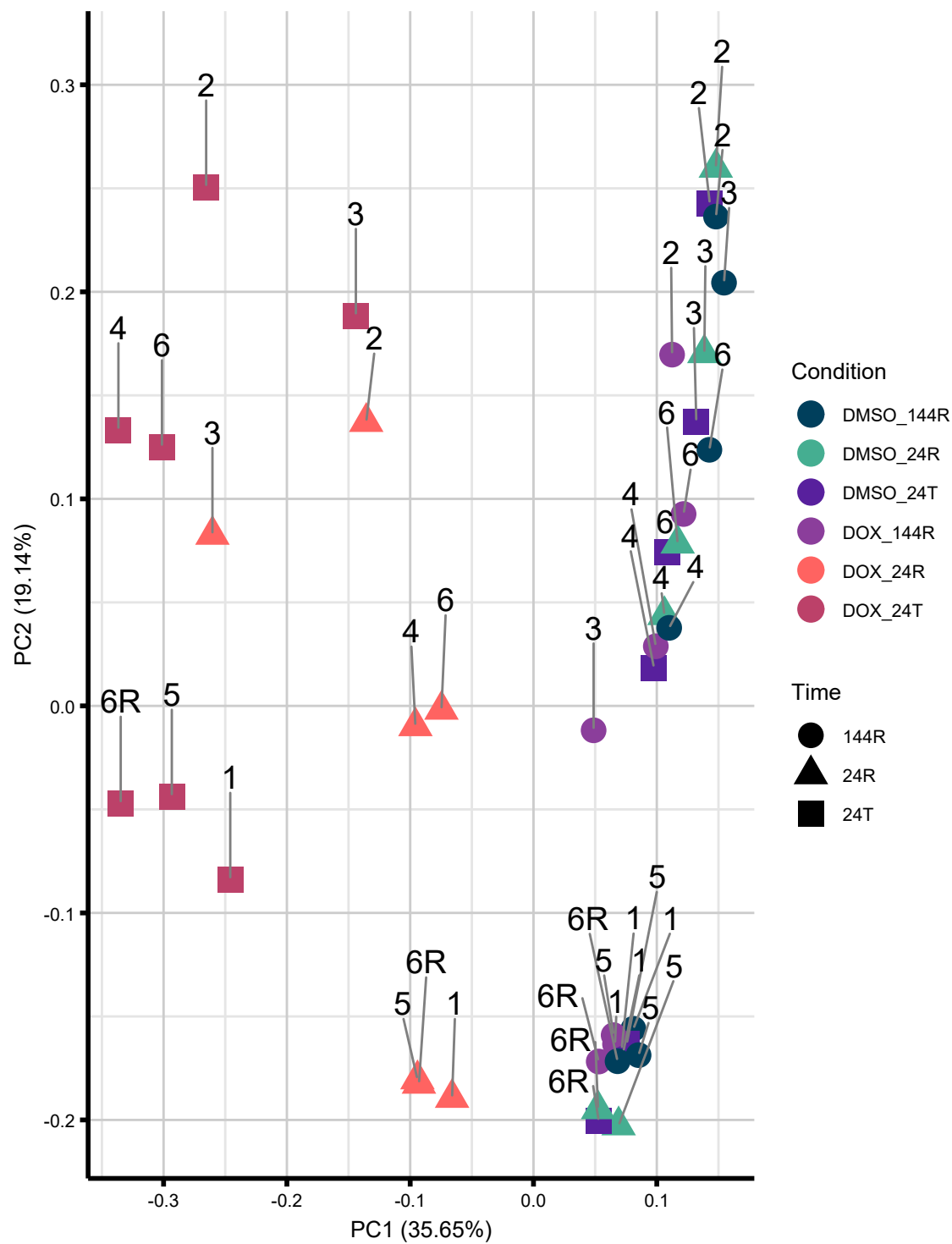
PCA of global gene expression (pre-RUV)
