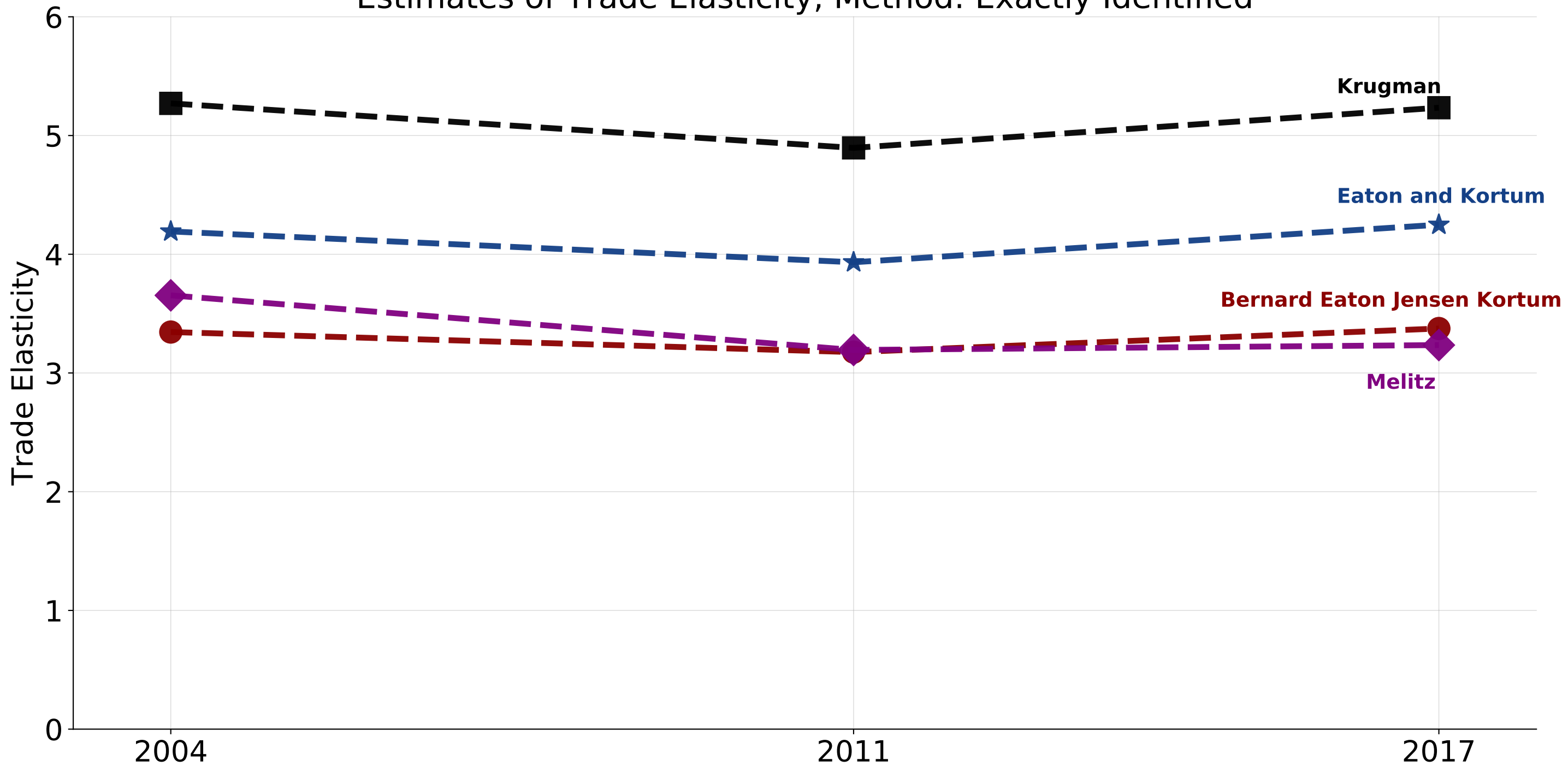
Estimates of Trade Elasticity, Method: Exactly Identified
