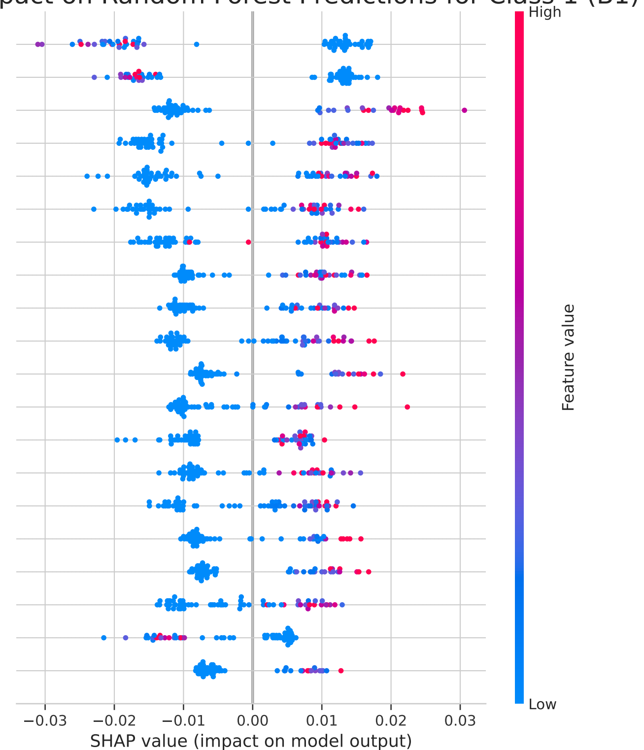
Feature Impact on Random Forest Predictions for Class 1 (B1)
