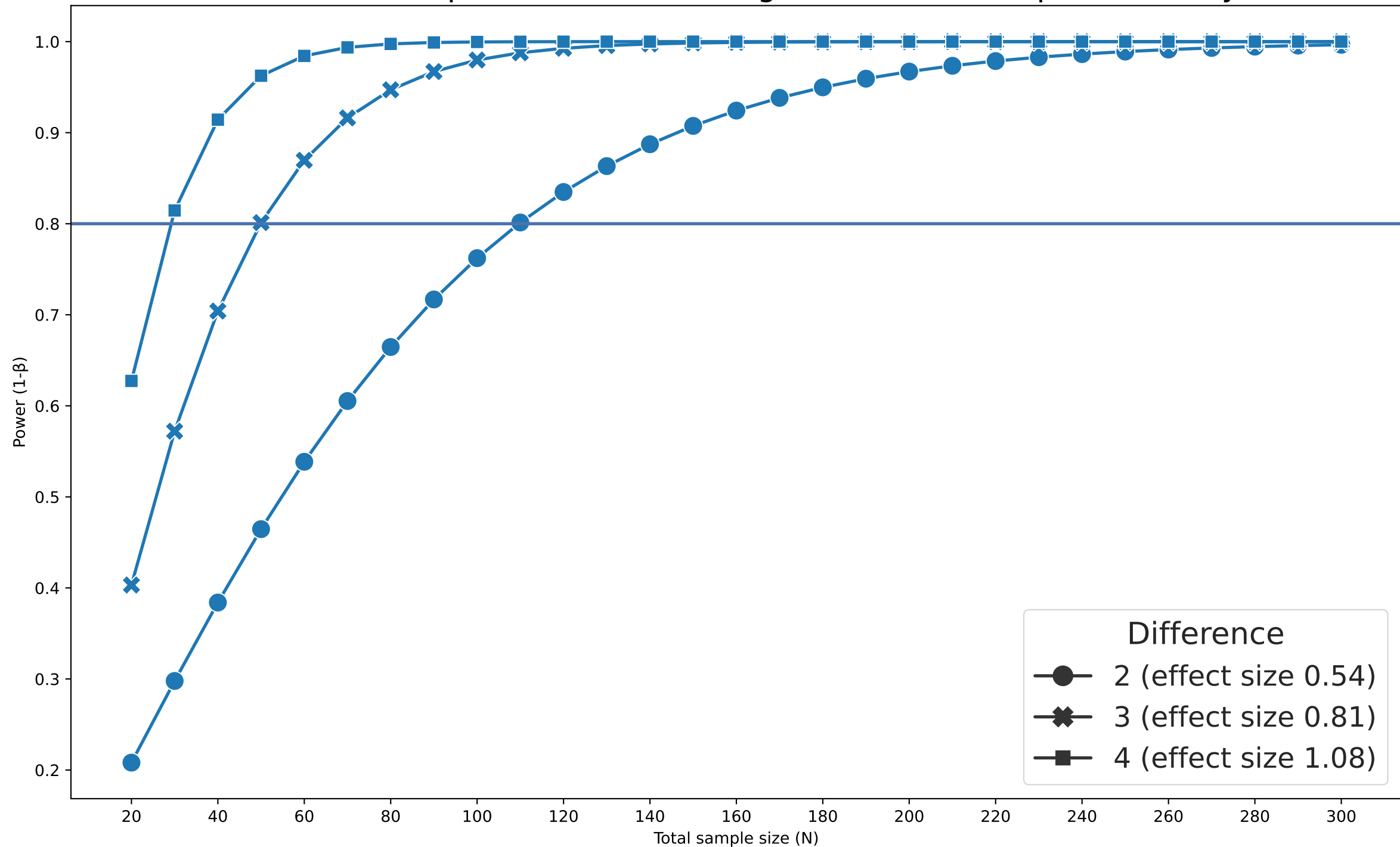
Power vs Sample Size for Detecting Differences in Alpha Diversity
