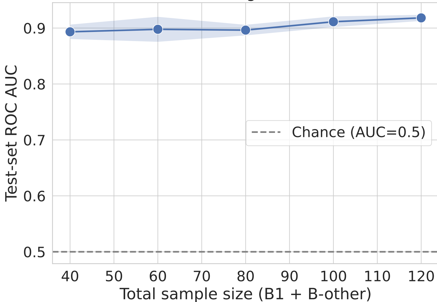
Random Forest learning curve: B1 vs B-other
