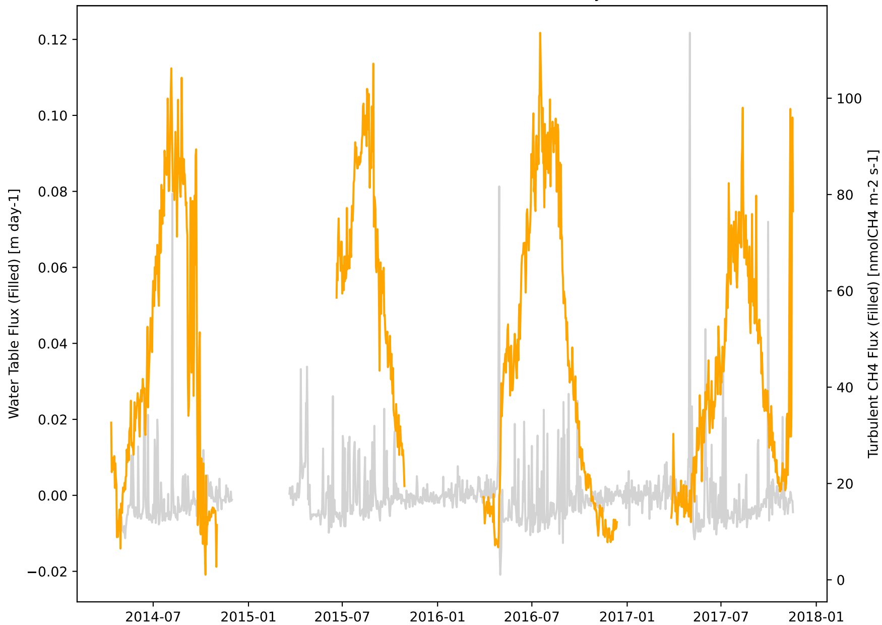
CA-SCB Site, WTD Flux and Methane Flux Dynamics
