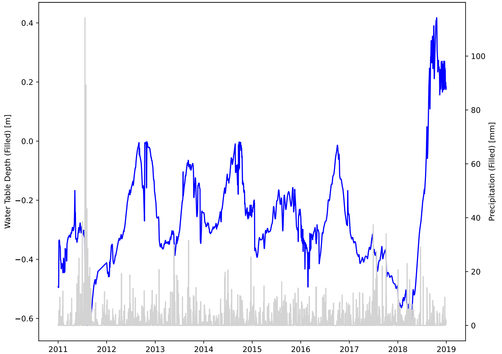
DE-Hte Site, Precipitation and WTD
