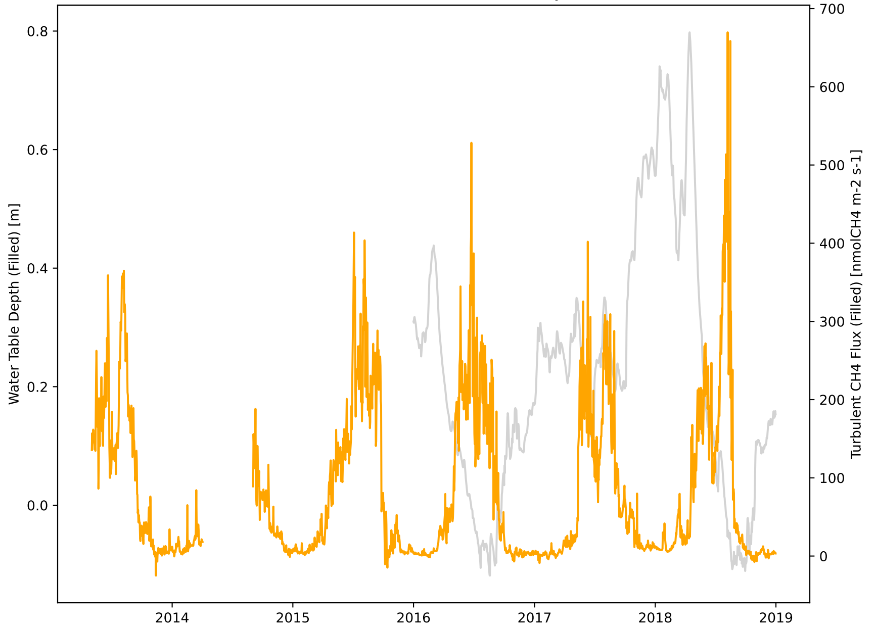
DE-Zrk Site, WTD and Methane Flux Dynamics
